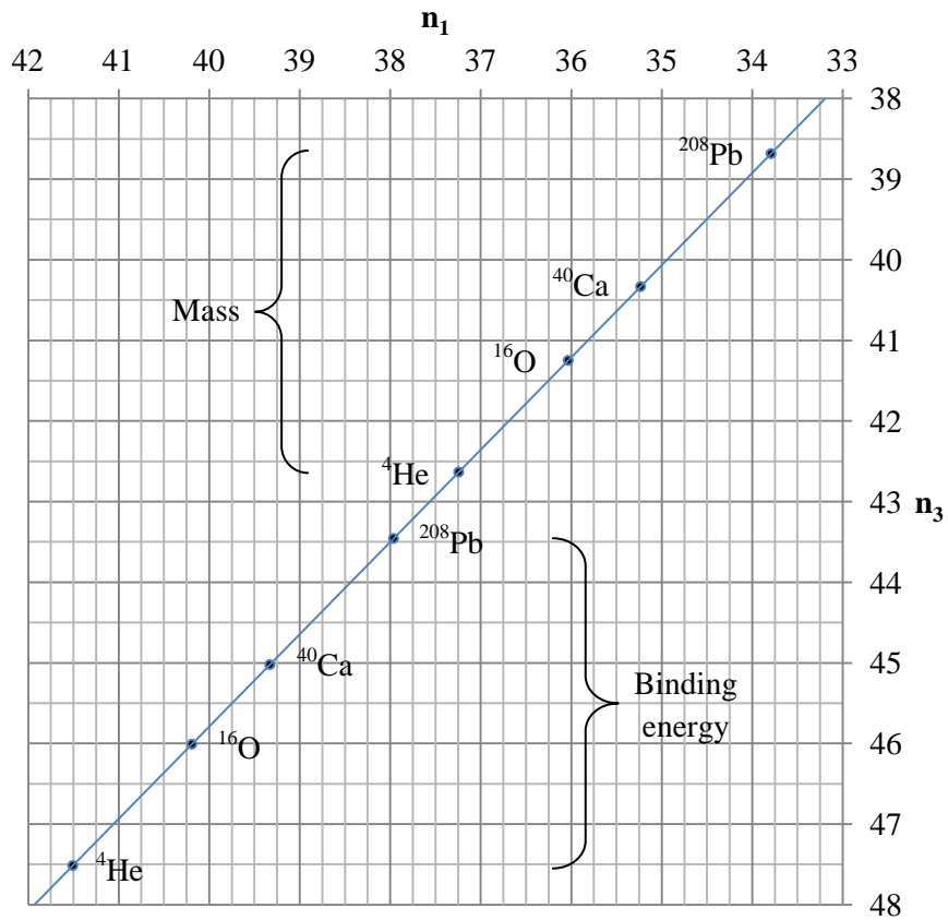
Figure 6: Masses and binding energies of four double magic number nuclei.
