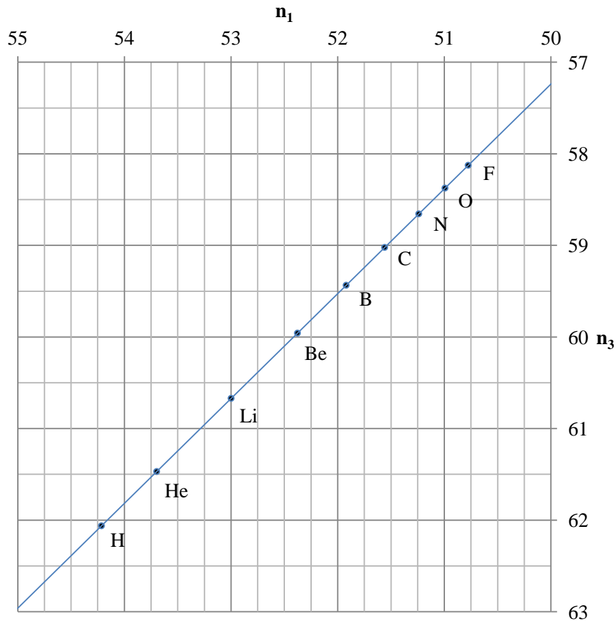
Figure 1: Electron K (1s) binding energies for the elements in their natural forms [6], in Sequences 1 and 3. The values of binding energy lie on a straight line since the level-numbers in Sequences 1 and 3 are in constant ratio.
