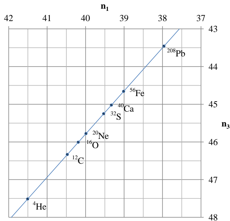
Figure 5: Binding energies of selected stable nuclei in Sequences 1 and 3.
