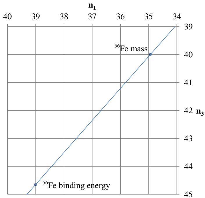
Figure 7: The mass and binding energy of the {}^{56}\text{Fe} nucleus within Sequences 1 and 3.
