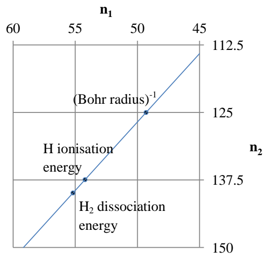
Figure 4: Hydrogen scales on the mass/energy levels of Sequences 1, 2 and 3.
