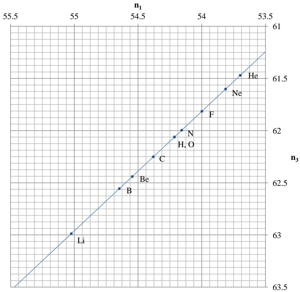
Figure 3: Ionisation potentials of the neutral atoms with Z = 1 to 10 [7], in Sequences 1 and 3.
