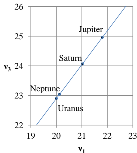
Figure 9: Gravitational binding energies of the gas giant planets of the Solar System on the trans-Planckian levels of Sequences 1 and 3.
