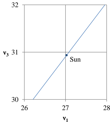
Figure 8: Gravitational binding energy of the Sun on the trans-Planckian levels of Sequences 1 and 3.
