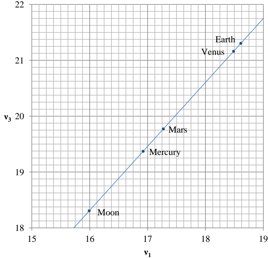
Figure 12: Gravitational binding energies of the rocky planets of the Solar System, and the binding energy of the Moon, on the trans-Planckian levels of Sequences 1 and 3.
