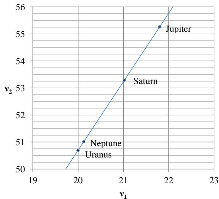
Figure 11: Gravitational binding energies of the gas giant planets of the Solar System on the trans-Planckian levels of Sequences 1 and 2.
