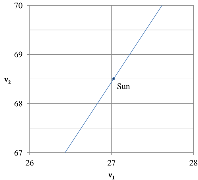
Figure 10: Gravitational binding energy of the Sun on the trans-Planckian levels of Sequences 1 and 2.
