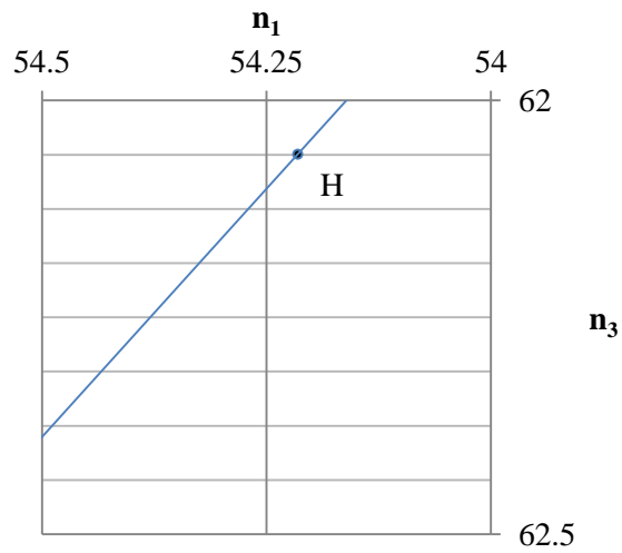
Figure 2: Detail of the hydrogen K (1s) binding energy, in Sequences 1 and 3.
