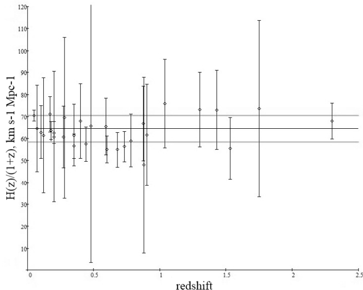
Figure 11: The ratio H(z)/(1+z) \pm \sigma and the weighted value of the Hubble constant \langle H_0 \rangle \pm \sigma_0 (horizontal lines). Observed values of the Hubble parameter H(z) are taken from Table 1 of [18] and one point for z < 0.1 is taken from [19].
