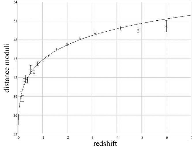
Figure 10: The theoretical Hubble diagram \mu_0(z) of this model (solid); quasar observational data (18 binned points) [16], corrected for no time dilation.
