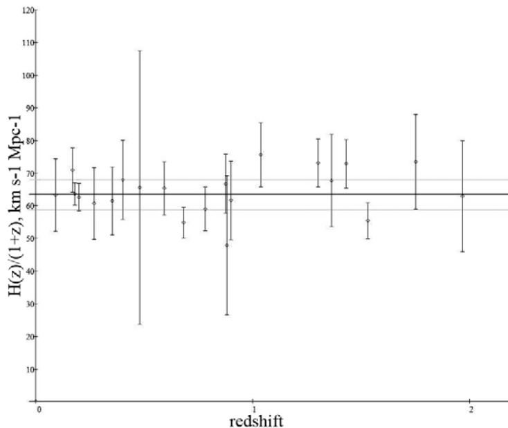
Figure 12: The ratio H(z)/(1+z) \pm \sigma and the weighted value of the Hubble constant \langle H_0 \rangle \pm \sigma_0 (horizontal lines). Observed values of the Hubble parameter H(z) are taken from [20].
