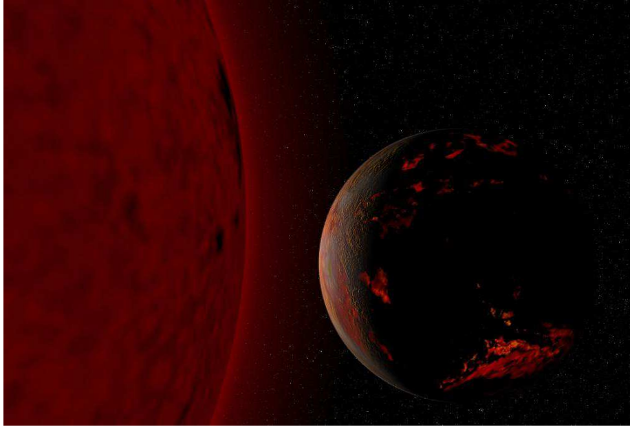
Earth in 5-7 billion years from now. Since we don't use this theory in application in next 1 billion years, oceans begin to evaporate
