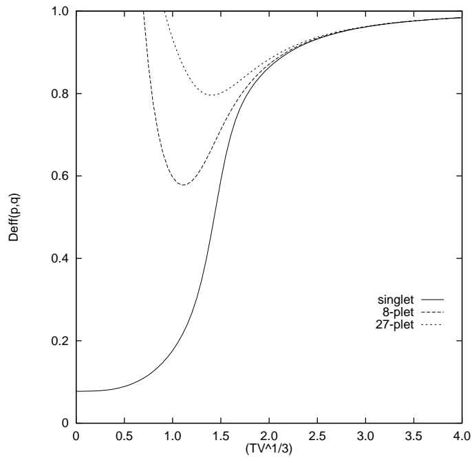
Figure 1: D_{eff}(p, q) for different colour representations : singlet, 8-plet and 27-plet as a function of TV^{1/3}/\hbar c . These results are for two-flavours.
