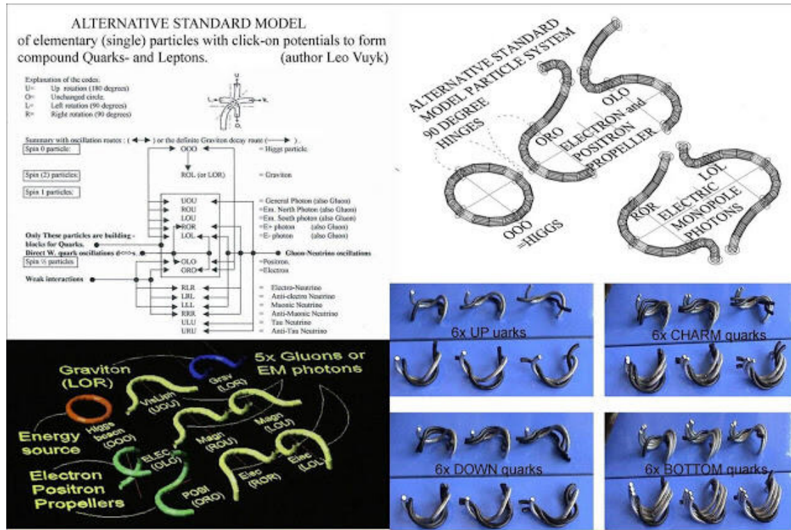
Figure 14. Quantum Particle system with adapted string shapes constructed out of only one torus Higgs mother particle.
