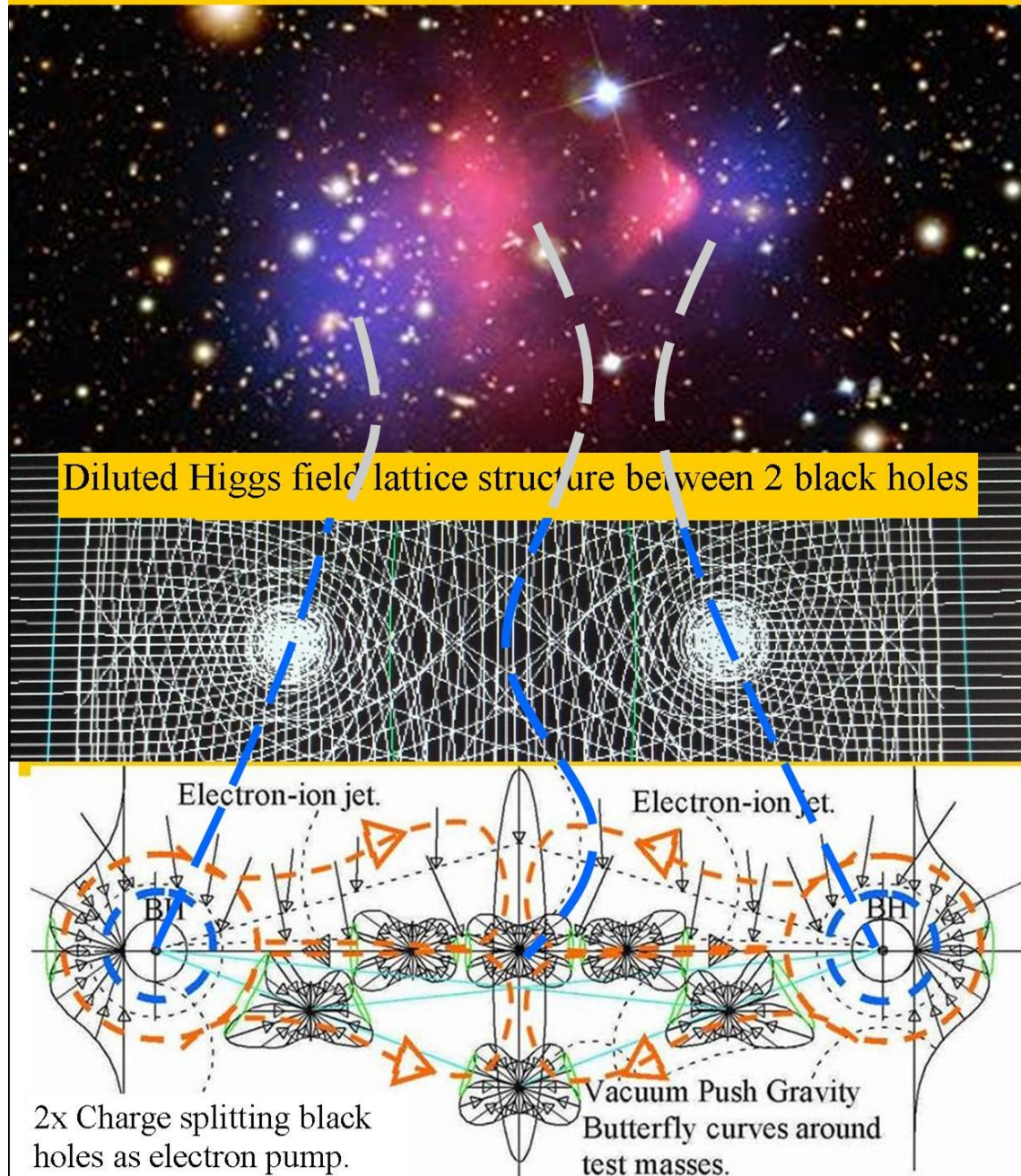
Figure 13 Diluted Higgs field vacuum space between two electric dark matter black holes or between dual Galaxy Anchor black hole systems.
