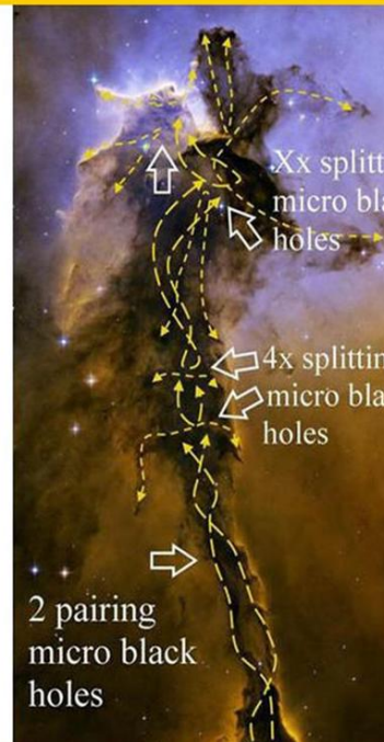
Figure 10, Yellow balls observed as early stars forming the center of open star cluster between two Herbig Haro black hole objects. In comparison with the Herbig Haro formation inside the Eagle nebula.
