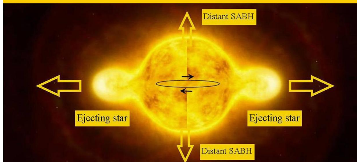
Figure 6, BOK globule with the proposal for symmetrical multiplication of failed stars being assumed to be a copy of real star multiplication inside larger molecular clouds, after instable rotation.
