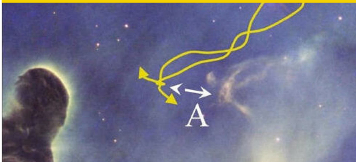
Figure 19, More examples of pairing and splitting micro black holes inside nebula to be formed into HH systems.
