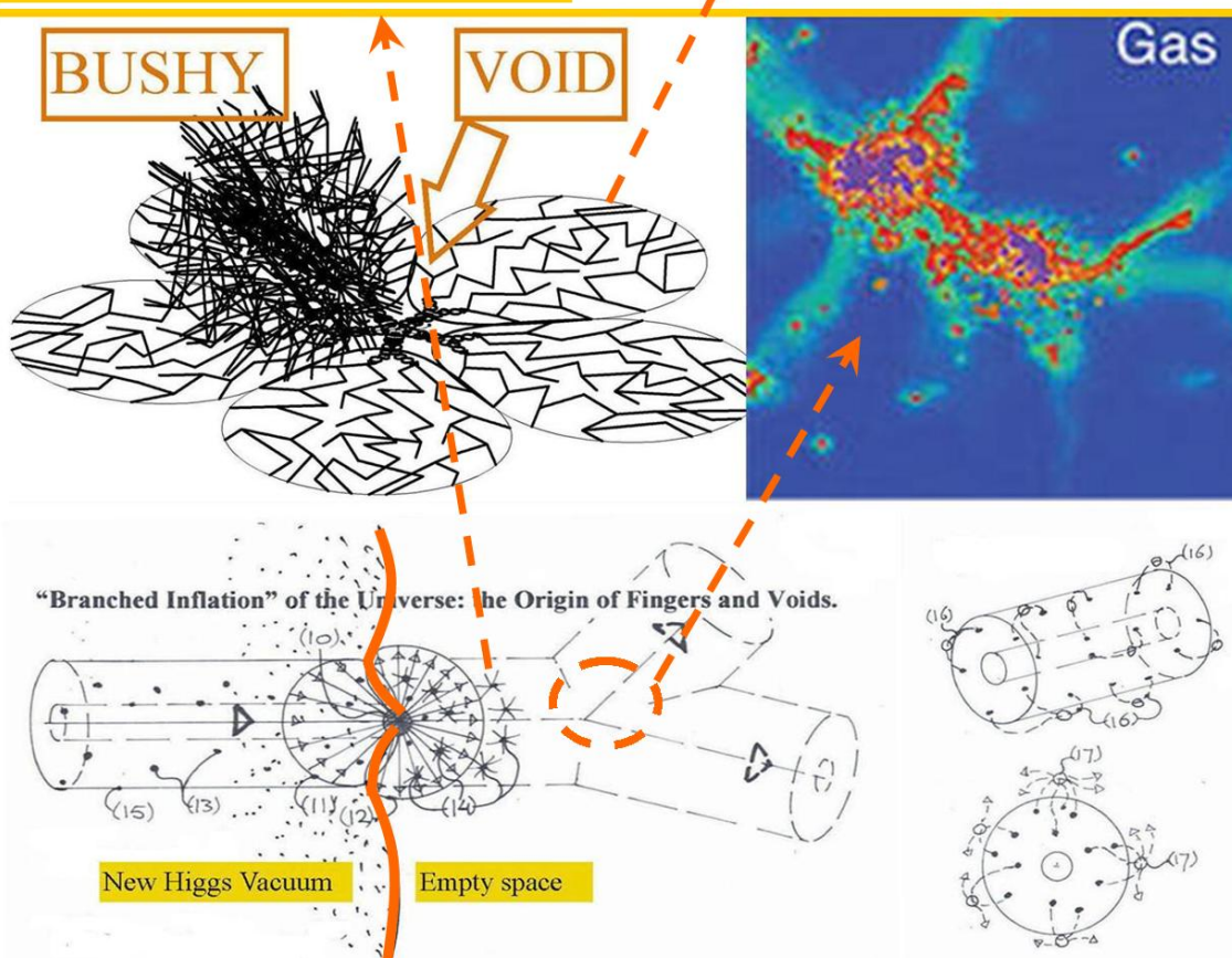
Figure 2. Splitting and pairing Big Bang splinter black holes are the origin of primordial star and Galaxy formation in combination with black hole evaporating into the Higgs vacuum.
