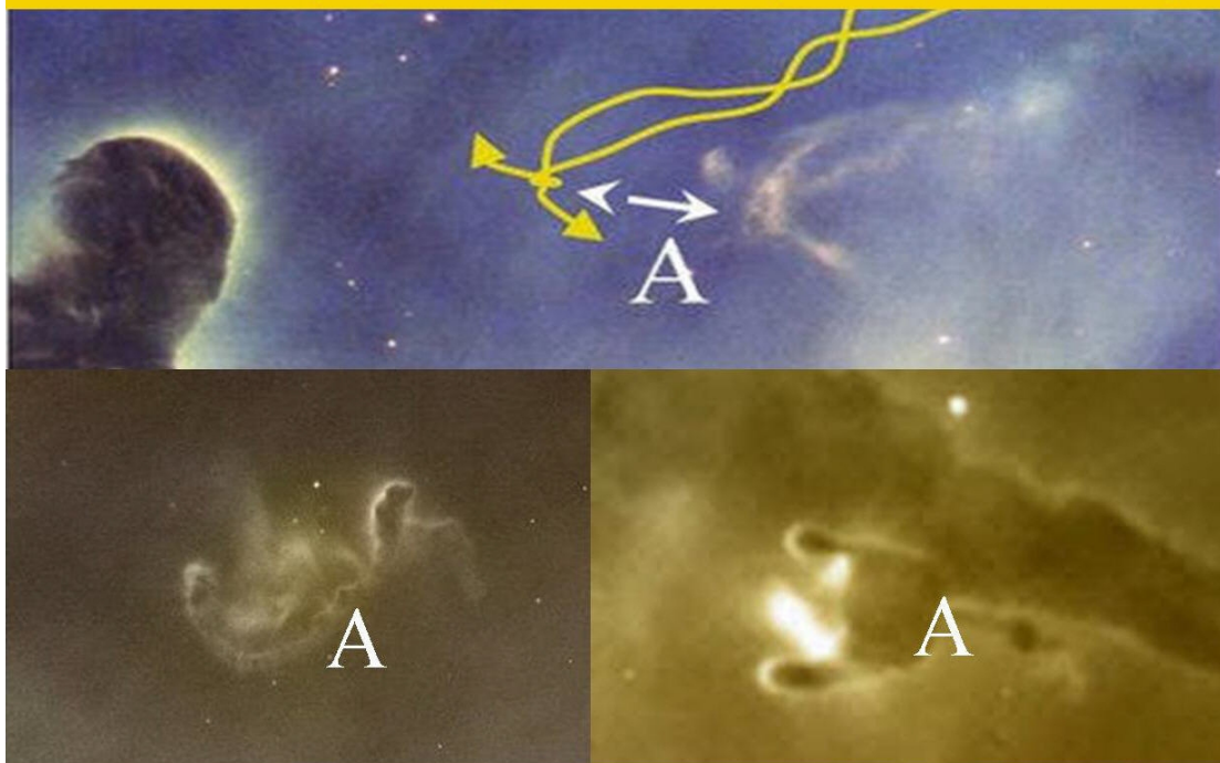
Figure 16. Examples of pairing and receding / splitting micro black holes inside nebula.
