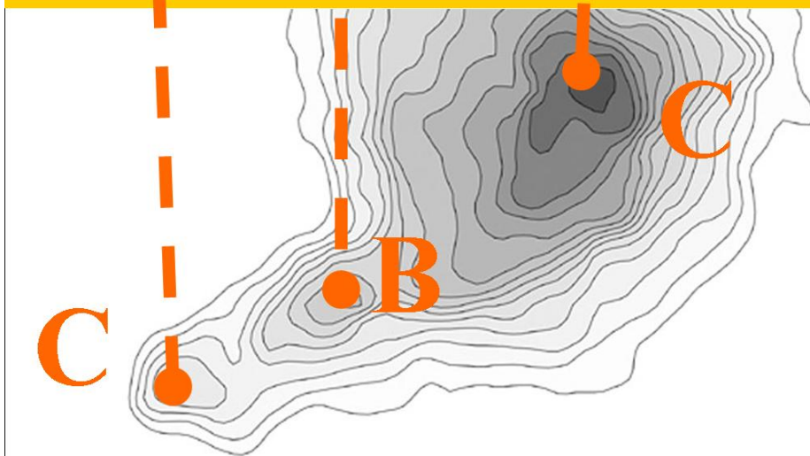
Figure 5, BOK globule density interior with proposal for dual black hole and white hole locations related to the production of so called “Failed Stars”.
