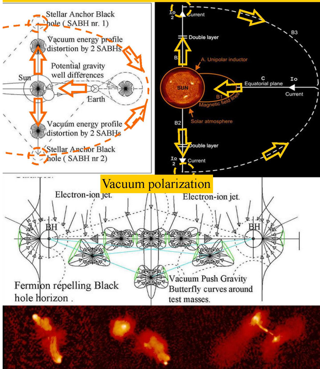
Figure 20. The solar system depicted as the result of a former Herbig Haro system.
