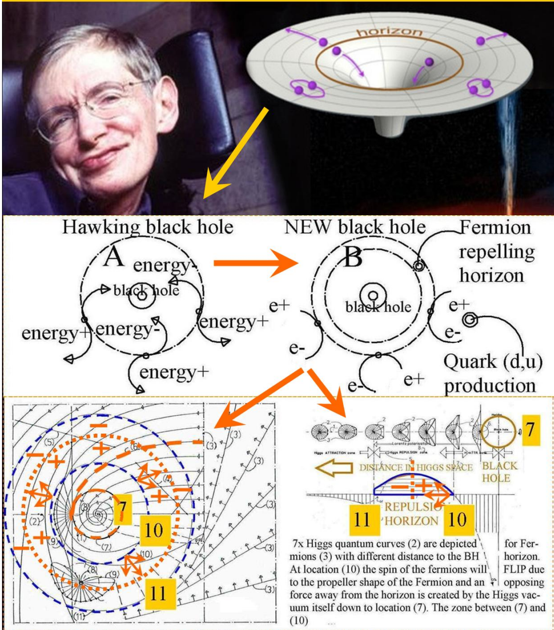
Figure 12, The difference between the mainstream Hawking black hole and the New BH of Quantum FFF Theory.
