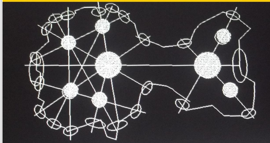
Figure 8, Micro black holes, being the expelled Starspots of exploding Nova stars, (Helix nebula) as the seedlings of Cometary nuclei such as Comet 67P.
