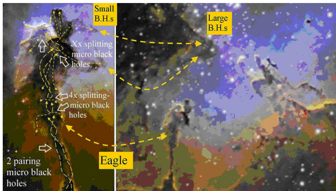
Figure 16. Examples of pairing and receding / splitting micro black holes inside nebula.
