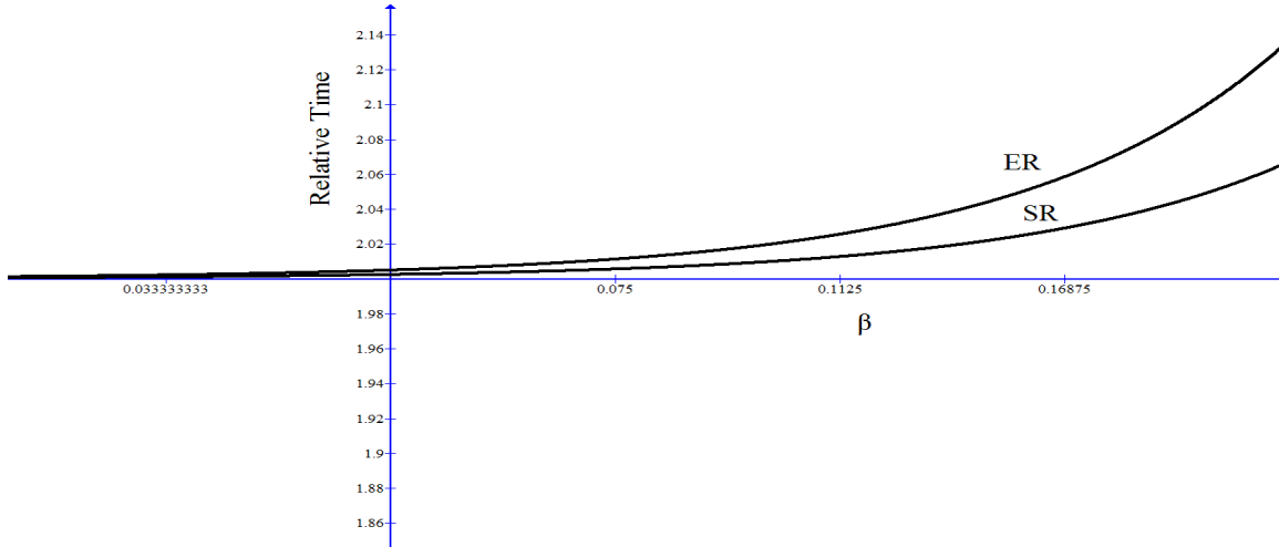
Figure 4: predictions of SR and ER for relatively low velocities
