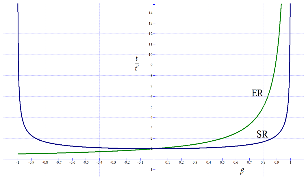
Figure 1: Time transformation in ER and SR
