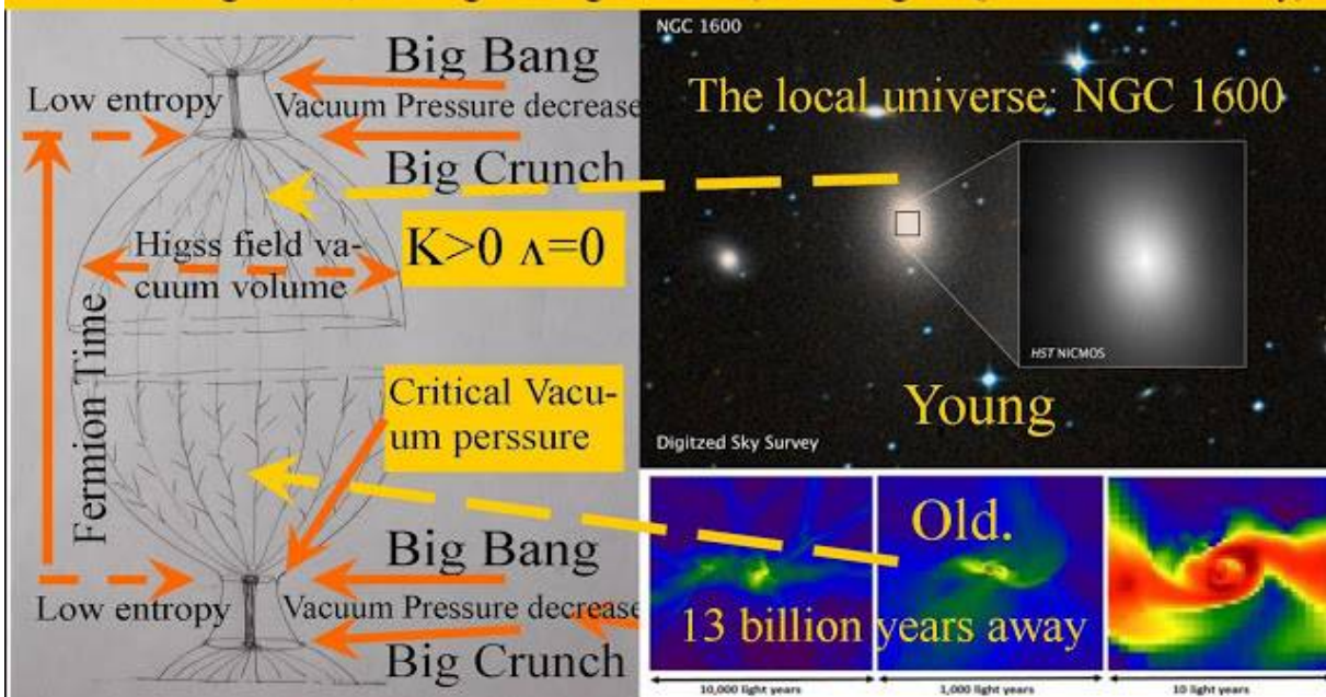
Figur 2. Imaging the cyclic multiverse. according to Quantum FFF Theory
