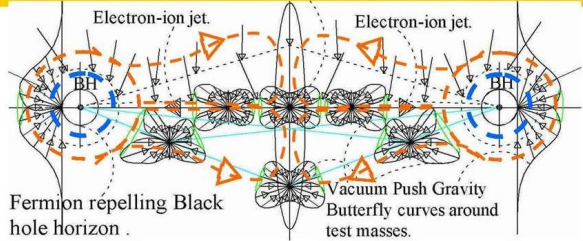
Figure 18, Birkeland and Alfvén current circuits around galaxies and Herbig Haro systems, for quick star formation in the centre.
