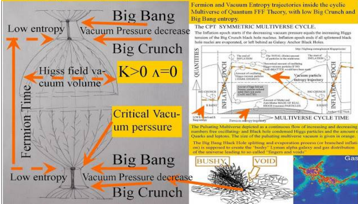
Figur 1. Imaging the cyclic multiverse, according to Quantum FFF Theory.
