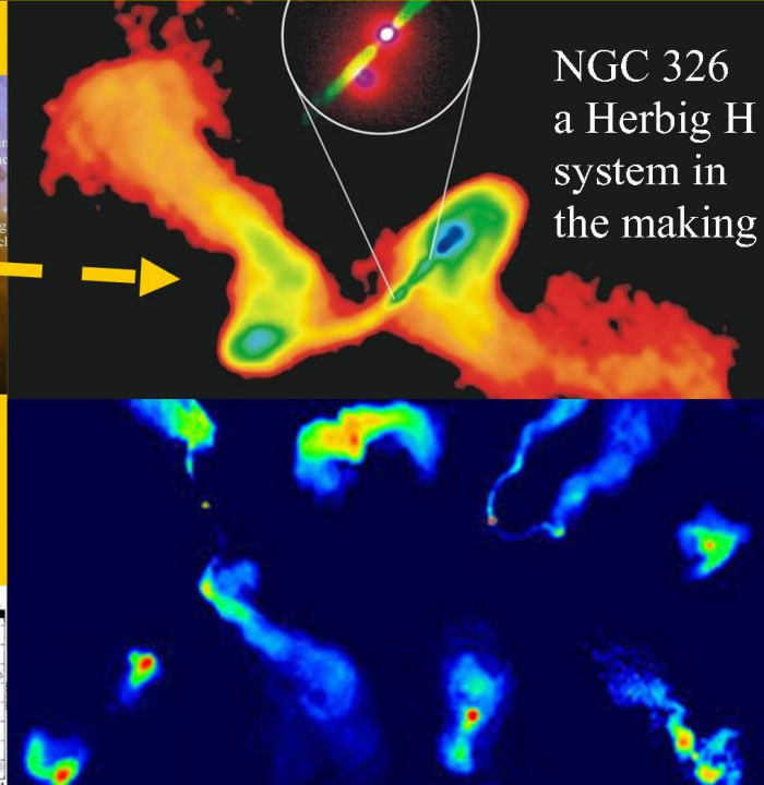
Figure 14 Plasma production around Herbig Haro objects and early galaxy Anchor Black Holes (GABHs).
