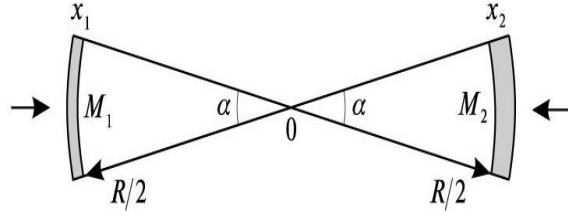
Fig. 2. Masses M_1 and M_2 in the form of ball segments with different thickness and matter density, located at the distance R from each other
