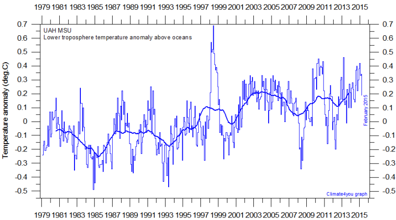
Fig.1. Global monthly average lower troposphere temperature above oceans since 1979,
