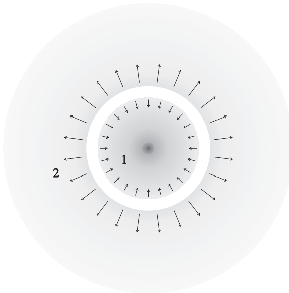
Fig. 1.— Separation of the pre-solar nebula into (1) a central spherical gas nebula and (2) an expanding spherical shell.
