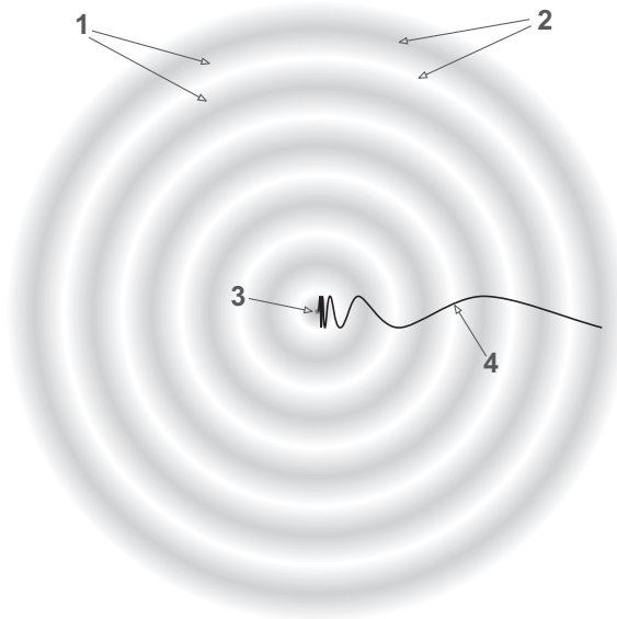
Fig. 2.— The standing wave in the pre-solar nebula: (1) nodes, (2) antinodes (gas compression and expansion), (3) protosun, (4) real-scale wave. Nodes and antinodes are evenly spaced for illustration purposes; in reality, separations would increase dramatically with increasing distance from the centre.
