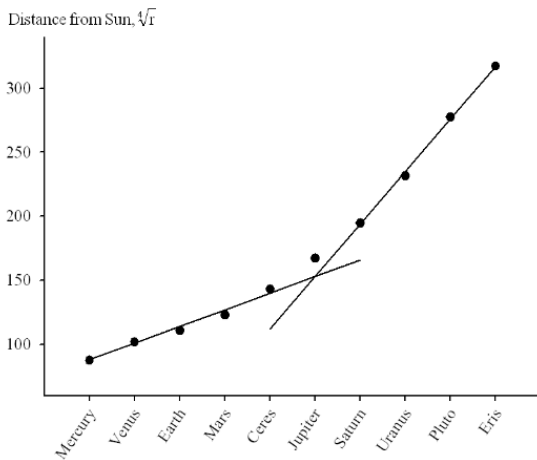
Fig. 5.— Distribution of planetary distances from the Sun. The vertical axis shows the fourth root of distance in kilometres.
