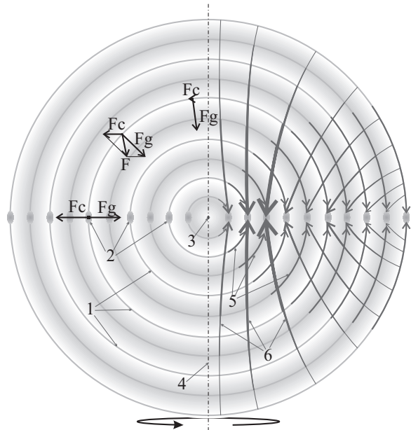
Fig. 3.— Migration of solid matter in the spherical nebula. F_g represents the gravitational pull toward the centre and F_c represents the centrifugal force. (1) spherical dust clusters in the antinodes, (2) dust clusters in the equatorial rings, (3) protosun, (4) nebula rotational axis, (5) direction of dust migration in the antinodes, (6) direction of massive dust cluster migration across the antinodes under the influence of the resultant force F .
