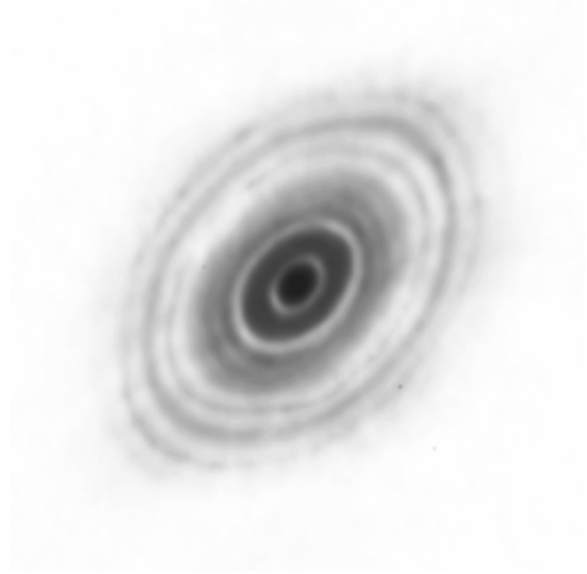
Fig. 4.— An image of a protoplanetary dust nebula around HL Tauri received by ALMA (The Atacama Large Millimeter/submillimeter Array), www.eso.org/public/images/eso1436a/
