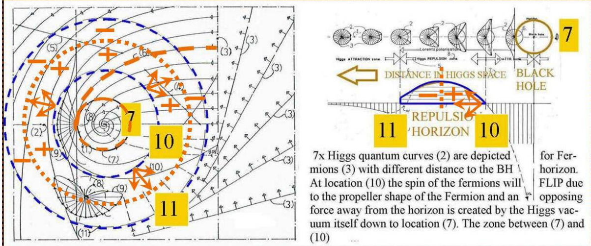
Figure 1, The new paradigm black hole.
