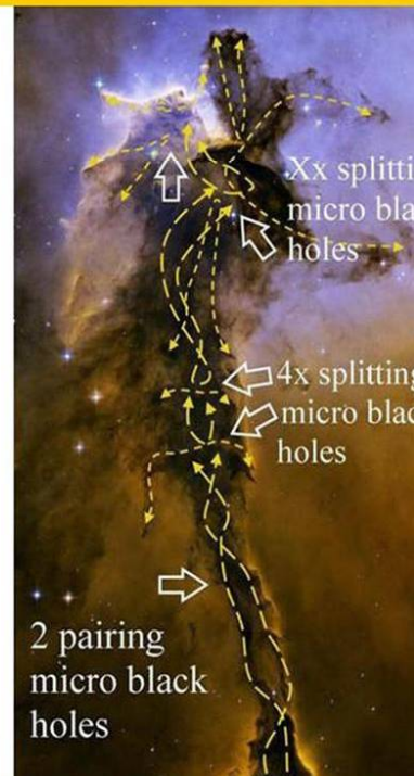
Figure 11, Yellow Balls as the start of Herbig Haro based Cepheid star production in open star clusters.
