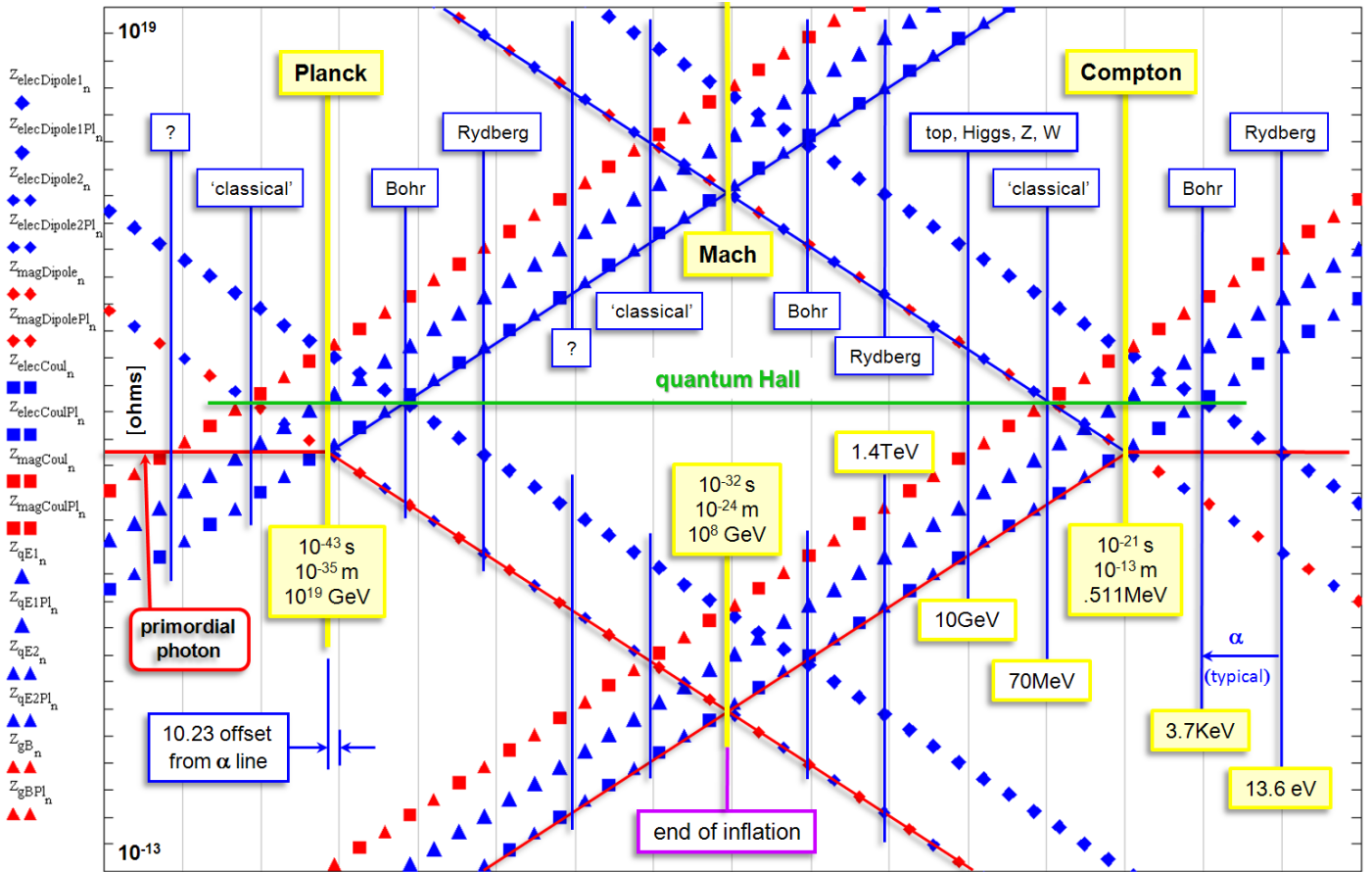
FIG. 3. A subset of the impedance networks of the Planck and Compton particles, showing both a .511 Mev photon entering from the right (included here not to imply relevance to the Big Bang but rather for illustrative purposes only), and the primordial photon entering from the left[16]. The end of inflation in the impedance approach (as in the Standard Model) comes at \sim 10^{-32} seconds, at the intersection of the two impedance networks, referred to here as the ‘Mach scale’.
