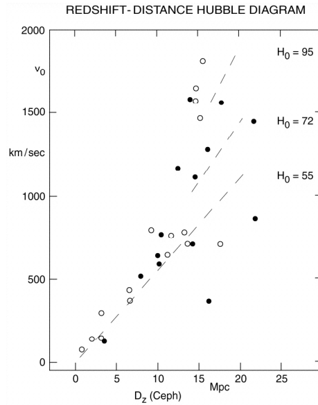
Figure 3: Hubble constants as a function of distance for Cepheids
