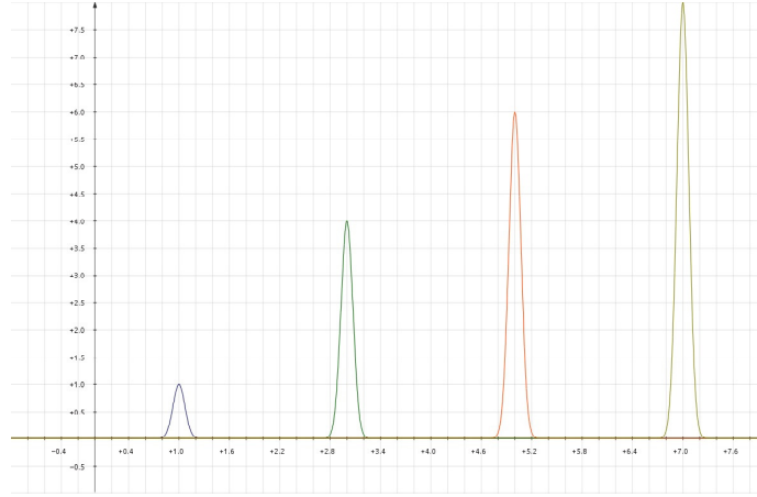
Figure 1: Spectral line evolution
