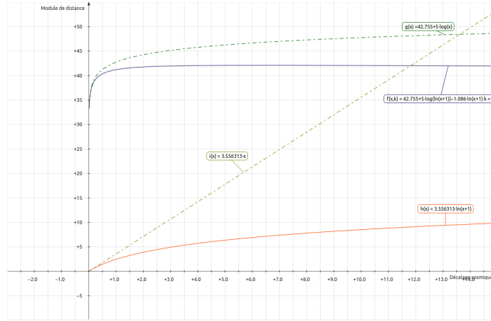
Figure 4: Distance modulus and true distance.
