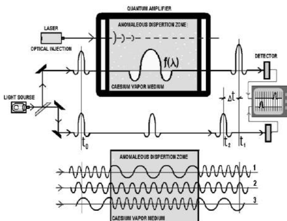
Fig. 5. Experiments of L.Wang - superluminal light propagation.
