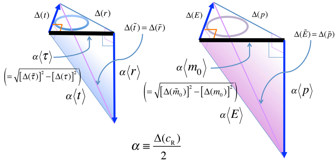
Figure 2. Vital to special relativity (SR) are both the (a priori constant) expectation value and the (event-observer specific) standard deviation of the speed of light . Observational statistics demands their coexistence. Featuring the uncertainty (or standard deviation) in the speed of light, stochastic SR leads to the two conjugate tetrahedrons as shown, with a) all facets being right-triangular and b) the nonzero \alpha scaling, into life, SR's two fundamental equations (shaded front facets) and all fundamental uncertainties. 'Classical' SR presumes zero \Delta(c_R) (or \alpha ), which erroneously entails that \Delta(t) = \Delta(r) and \Delta(E) = \Delta(p) , both valid only for massless particles, hold for mass entities—as evidenced by the two top facets, which vanish into a line segment for \langle \tau \rangle \neq 0 and \langle m_0 \rangle \neq 0 , as \alpha = 0 . Emphasizing the operational definition for the speed of light, stochastic SR rectifies the problem of 'classical' SR.
