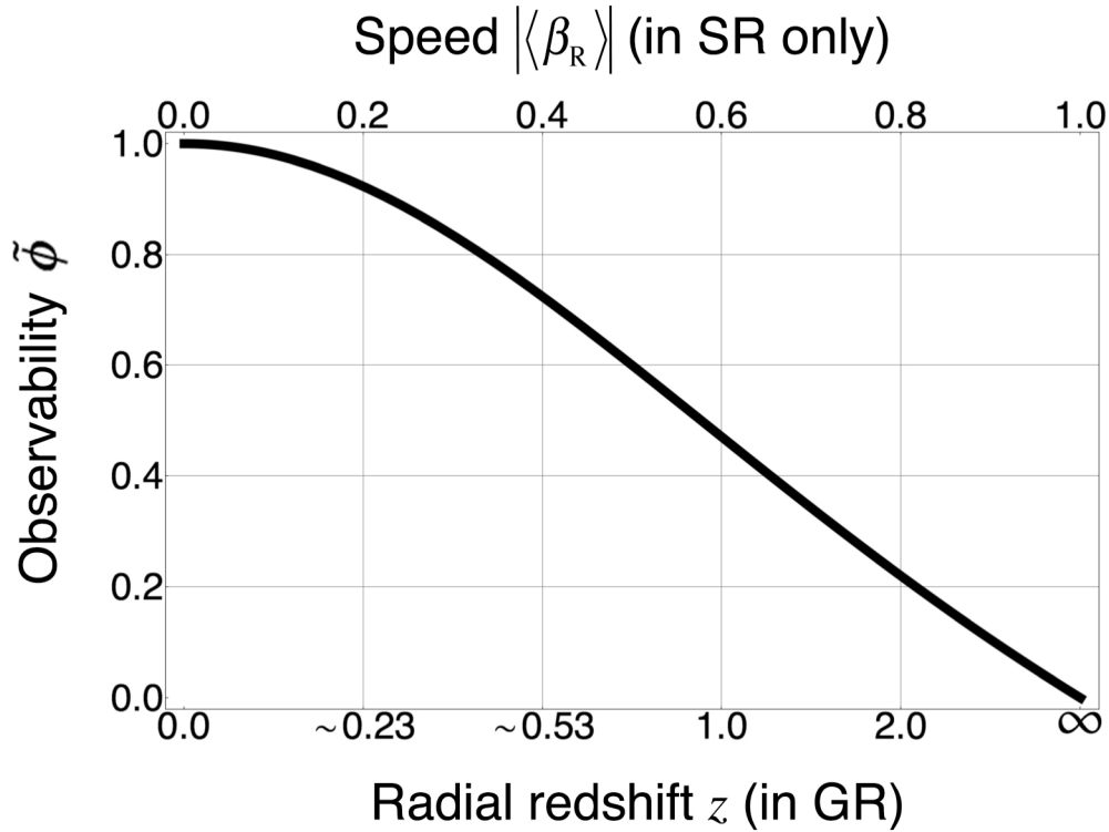
Figure 1. Blue- and redshift diminish event's observability \tilde{\phi} , namely, the relativistic quantum efficiency in observing the event . Independent of the (event-to-observer) luminosity distance, \tilde{\phi} is the (counterintuitive) observation-effectiveness of the event's luminosity, in emission of any elementary particle(s). In (stochastic) special relativity (SR), \tilde{\phi} varies with the radial speed |\langle \beta_R \rangle| (upper abscissa) of the event, per equation (6). In general relativity (GR) (and SR), \tilde{\phi} varies with the radial redshift z: (0, \infty) (lower abscissa) of the event's emission, per equation (12) after generalized in section 6. For the radial blueshift z: (-1, 0) , \tilde{\phi}(z) shows the same curve, but left-right reversed. Over the entire domain z: (-1, \infty) , \tilde{\phi}(z) —peaking at z=0 —is the universal resonance in the relative length-scale between the event and the observer (i.e., a subsequent event).
