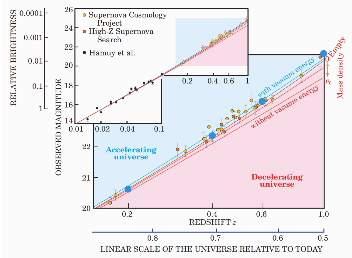
Figure 3. ‘Observed-magnitude [5] m vs. redshift z of Type Ia supernovae’ denies cosmic acceleration. (Other than the four blue dots, the figure along with the italicized original legend below is a reproduction with permission from Ref. [1], Copyright 2003, American Institute of Physics.) The original legend reads
