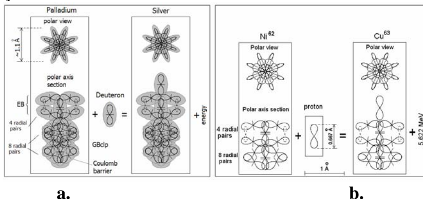
Fig. 13. a. - a nuclear reaction Pd + D → Ag [9] (the grey pattern shows the near Coulomb field), b. - a nuclear reaction Ni + H → Cu [13].
