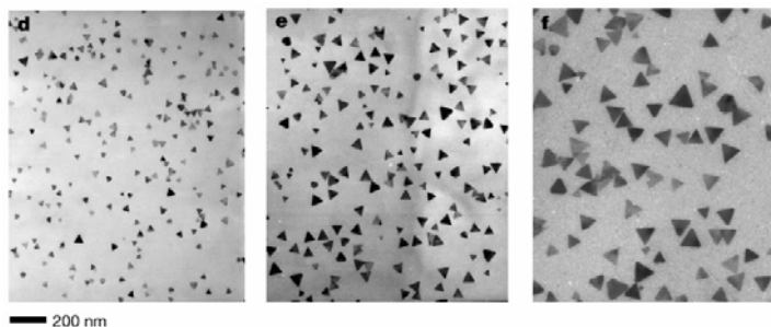
Fig. 17. Electron microscope image of silver nanoparticles. Courtesy of R. Jin et al. Nature 2003 [16]
