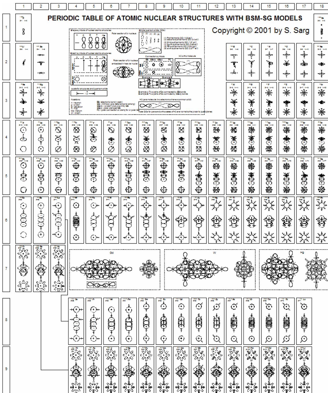
Fig. 20. Periodic table of nuclear atomic structures with BSM-SG atomic models, a poster included in the Atlas of Atomic Nuclear Structures [17,18,19]. For simplicity, the protons and neutrons are shown with symbolic graphical elements: proton - with an arrow and neutron with a line crossing the arrow.
