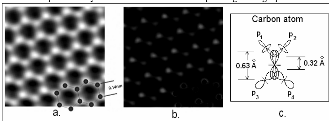
Fig. 15. a – image by TEAM microscope [15], b – processed image by brightness adjustment, c – carbon atom
