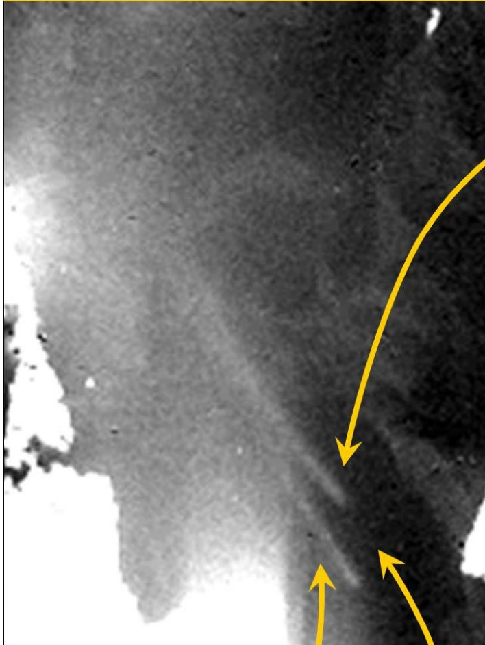
Central growth of single nuclear Comets and Coal. Comparison H 2 O perion, a moon of Saturn but assumed to be a former Comet, left alone by its dark matter black hole nucleus (Diameter about 300 km) with a Coral structure. (Right image, diameter a few mm). According to Quantum FFF Theory.
