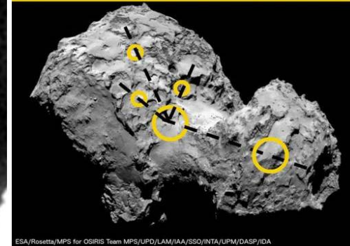
Comet 67P Craters originated by aligned gravity point sources according to Quantum FFF Theory.
