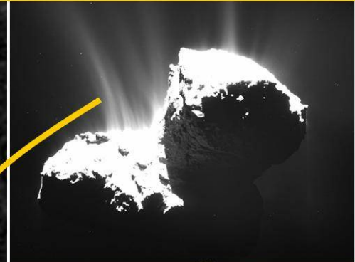
Comet 67P Craters originated by aligned gravity point sources according to Quantum FFF Theory.
