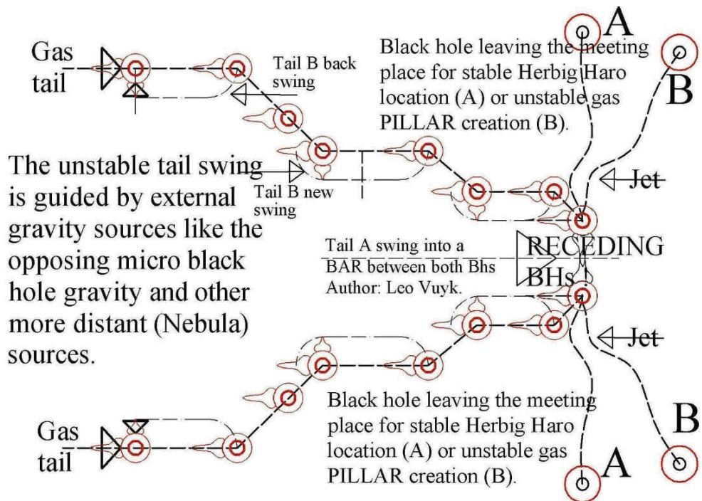
Figure 6, New Black hole propulsion principle by a self produced plasma-dust tail,. As a consequence, New black holes do not merge to form larger nuclei, they even repel negative charged metal surfaces by their own exterior electron charge. ( see also fig. 9)
