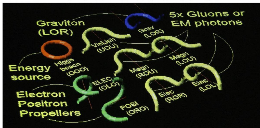
Figure 10, The particle zoo of single ELEMENTARY particles made out of ONE convertible Torus shaped Higgs particle, equipped with three hinges of 90 degree rotation.
