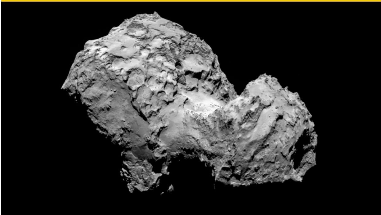
Figure 12: Dumbbell shaped Comets, 25 Hartley and Comet 67P C-G.
