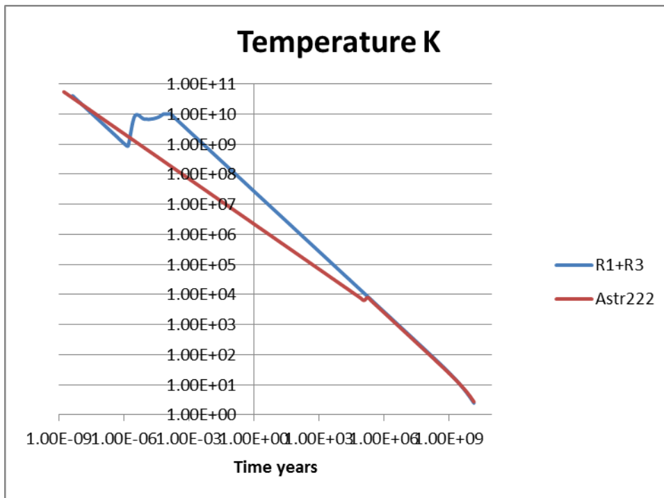
Figure 4:17 Expansion Temperature History including He4 Fusion
