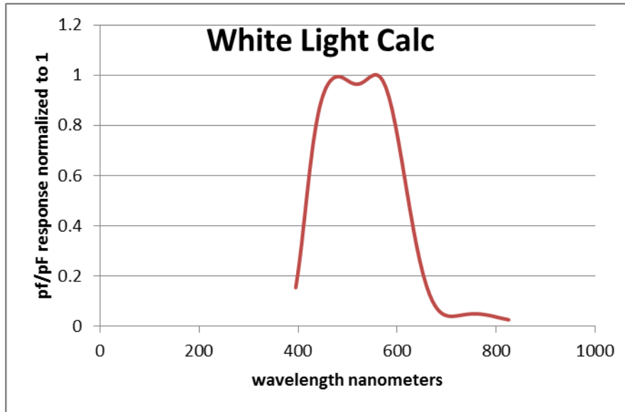
Figure 6:8 Adding Equal Color Responses Produce White Light
