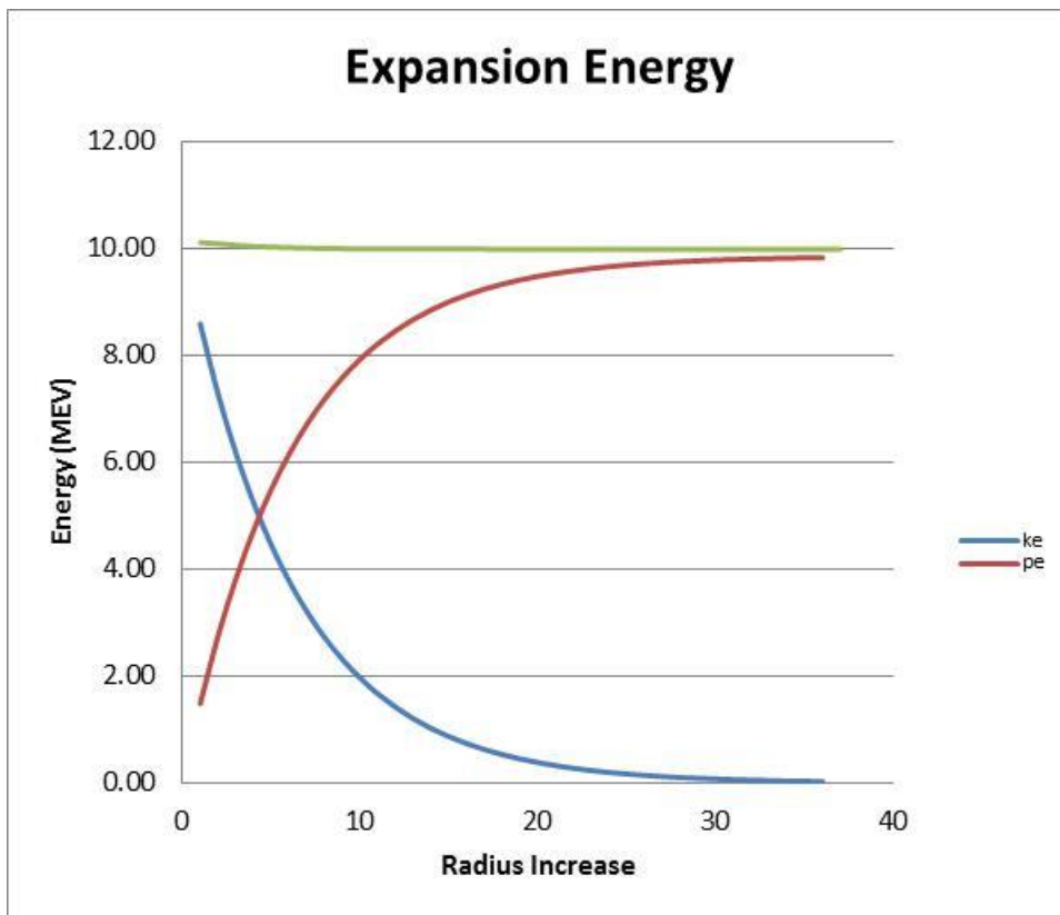
Figure 4:12 Conversion of Kinetic Energy to Kinetic Energy
