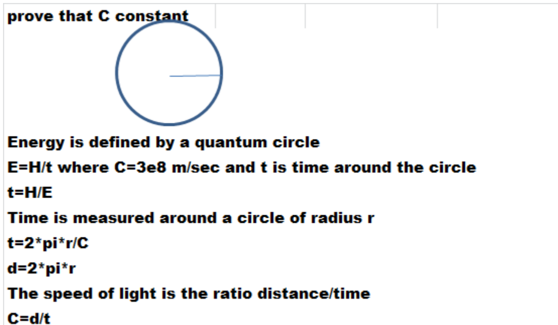
Figure 8:3 Why Light Speed is Constant
