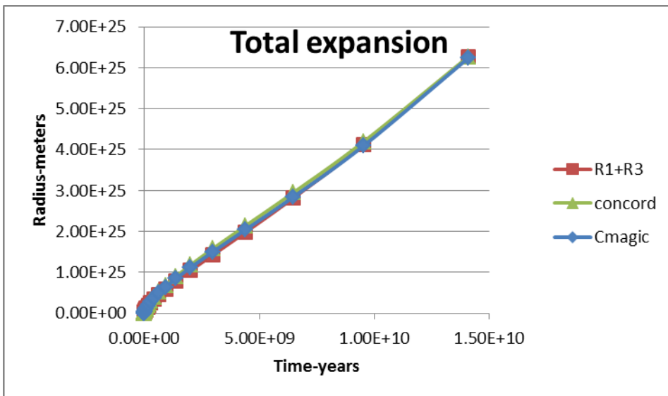
Figure 4:9 Total Expansion
