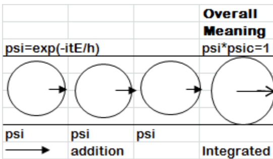
Figure 10:1 Repeat of Linked Probability Proposal
