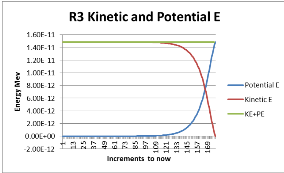
Figure 4:13 Dark Energy
