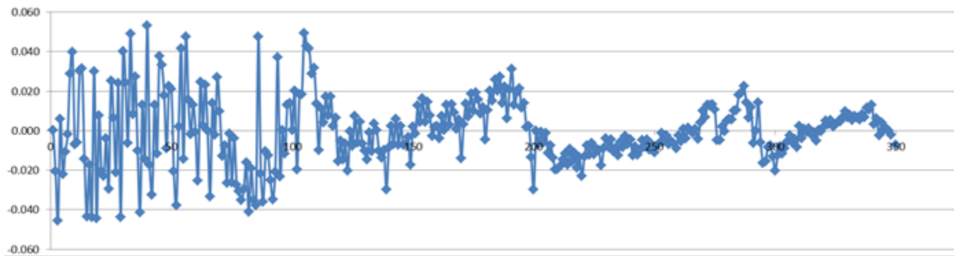
Figure 5:6 Binding Energy Accuracy (MeV)
