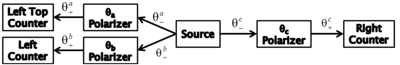
Figure 3. The triphoton experiment proposed in [2,3]
