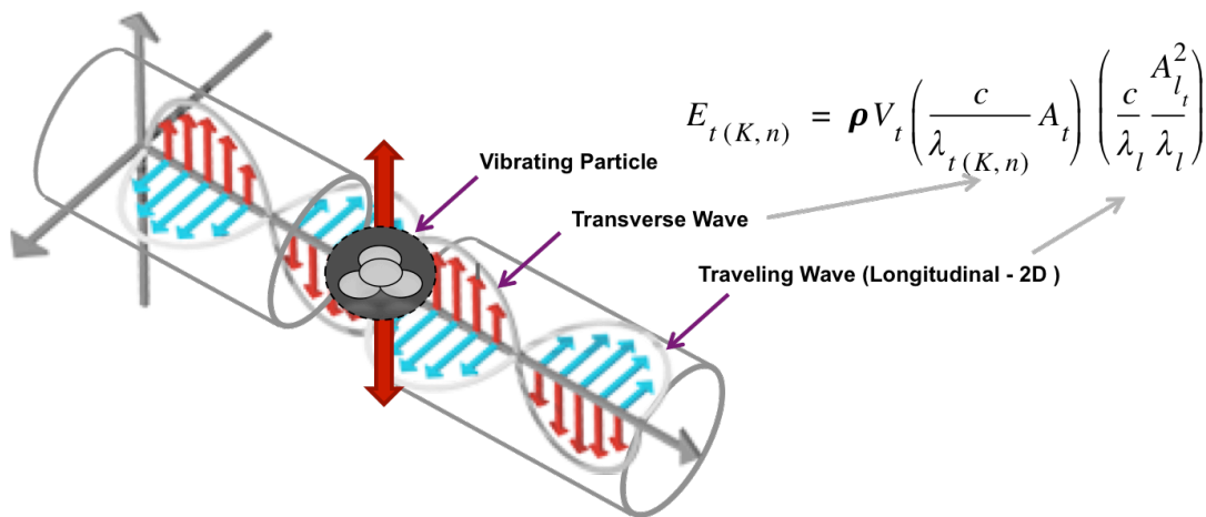
Fig 3.3.1 – Transverse Waves
