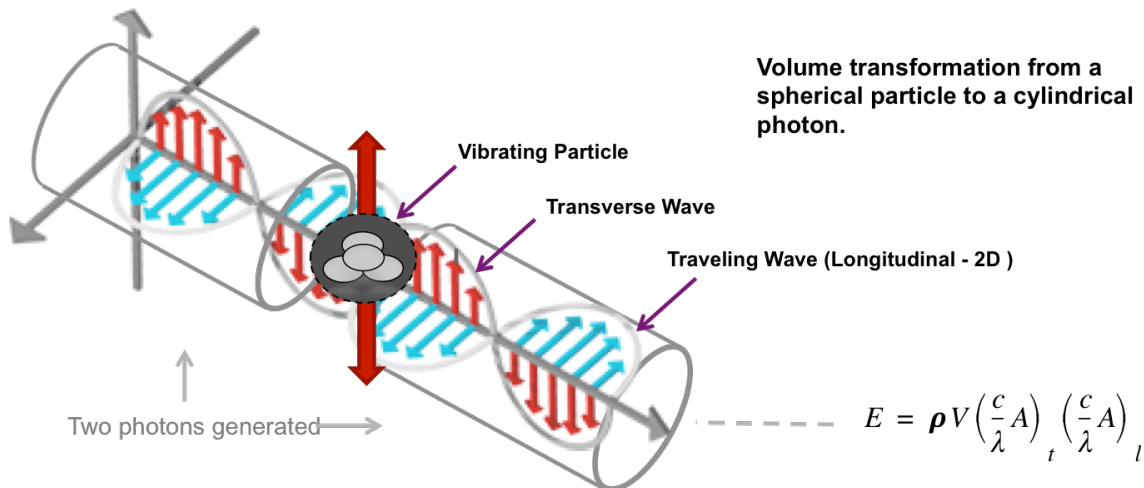
Fig 3.2 – Transverse Waves
