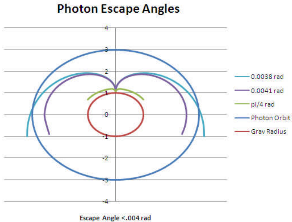
Figure 3. Illustration of the photon emission angle for photons that escape, and those photons that would be captured in orbit.
