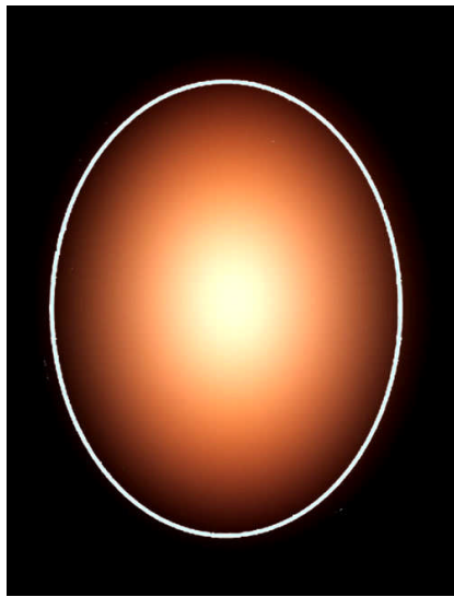
Figure 10. NDS: Simulated image of the escaping radiation from the Neutron Dark Star. The Full Width Half Maximum diameter is about 3.85 Schwarzschild radii. The white circle is the NDS shadow diameter of about 5.86 r_s
