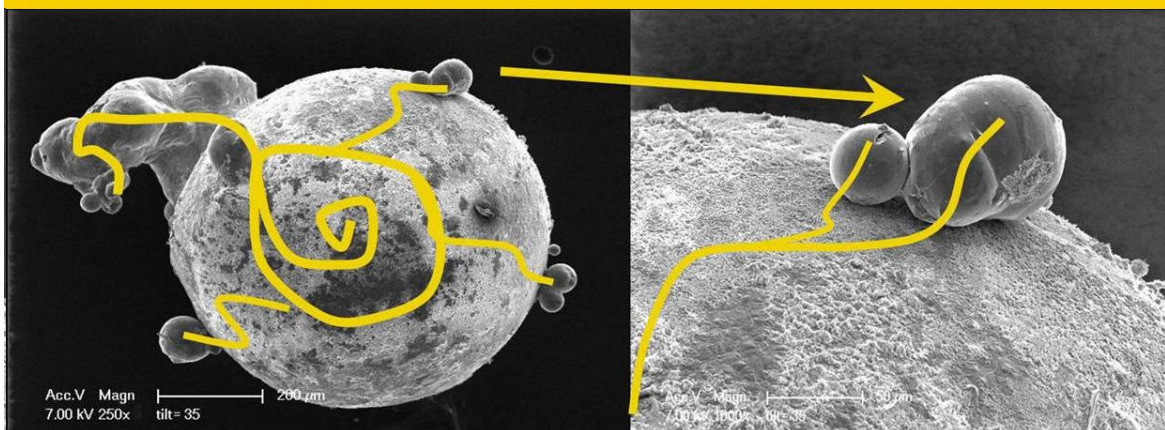
Figure: 13, Battery damage and UFO particles at CERN by dark matter (Quantum Knot) evaporating energy. Even stainless steel globules up to 3000 degr C. are possible ( Boeing 787 battery damage )
