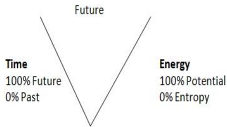
Fig. 3a Light cone at Big Bang
