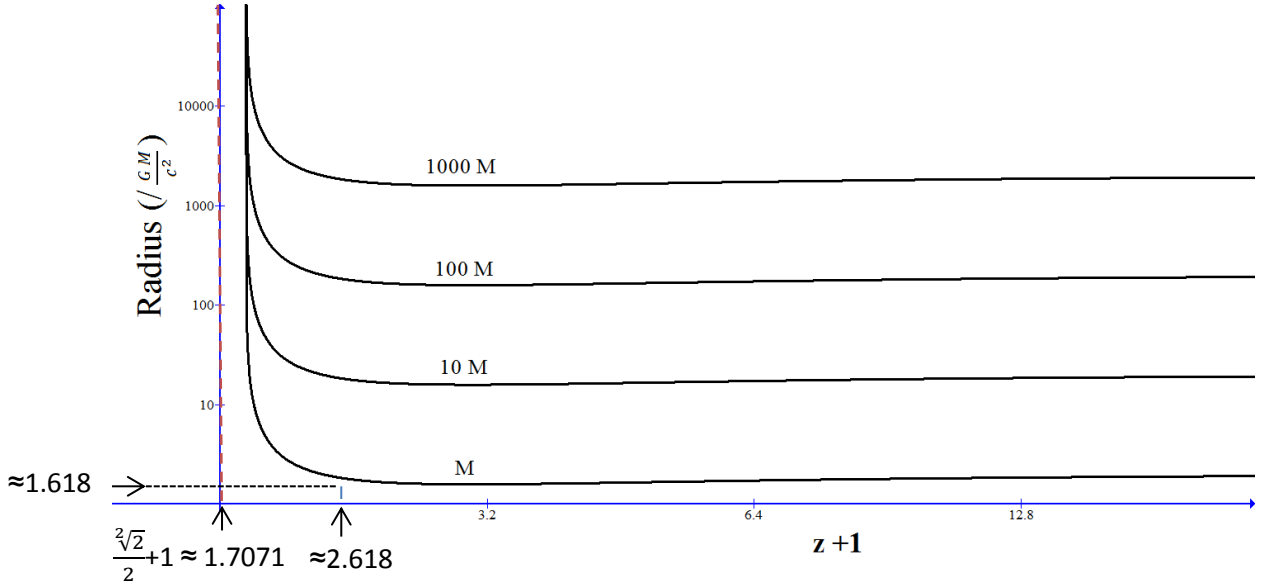
Figure 4 Radius as function of redshift
