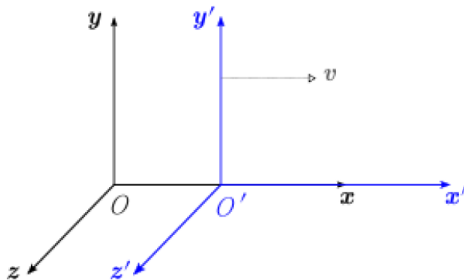
Figure a1. Observers in two reference frames moving with velocity v with respect to each other
