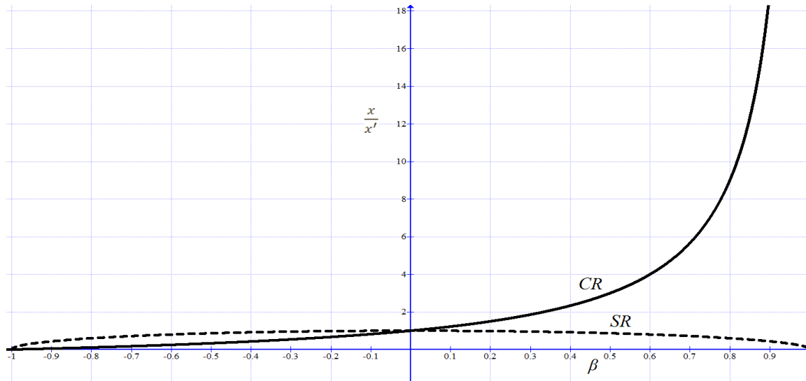
Figure a2. Distance transformation for the one-way trip. The dashed line depicts the corresponding prediction of SR
