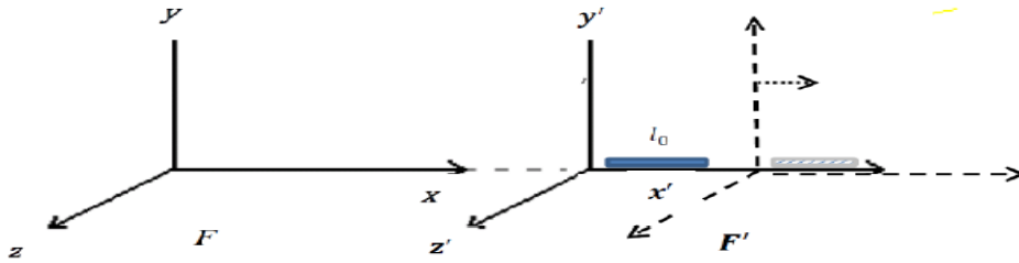
Fig. a4. Two observers in two reference frames, moving with constant velocity v with respect to each other
