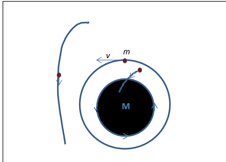
Figure 2 Three particles near a black hole
