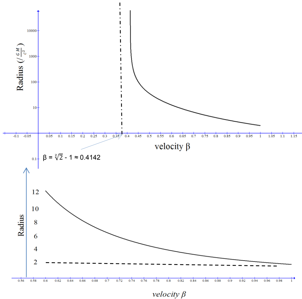
Figures 3a-3b Black hole radius as function of velocity
