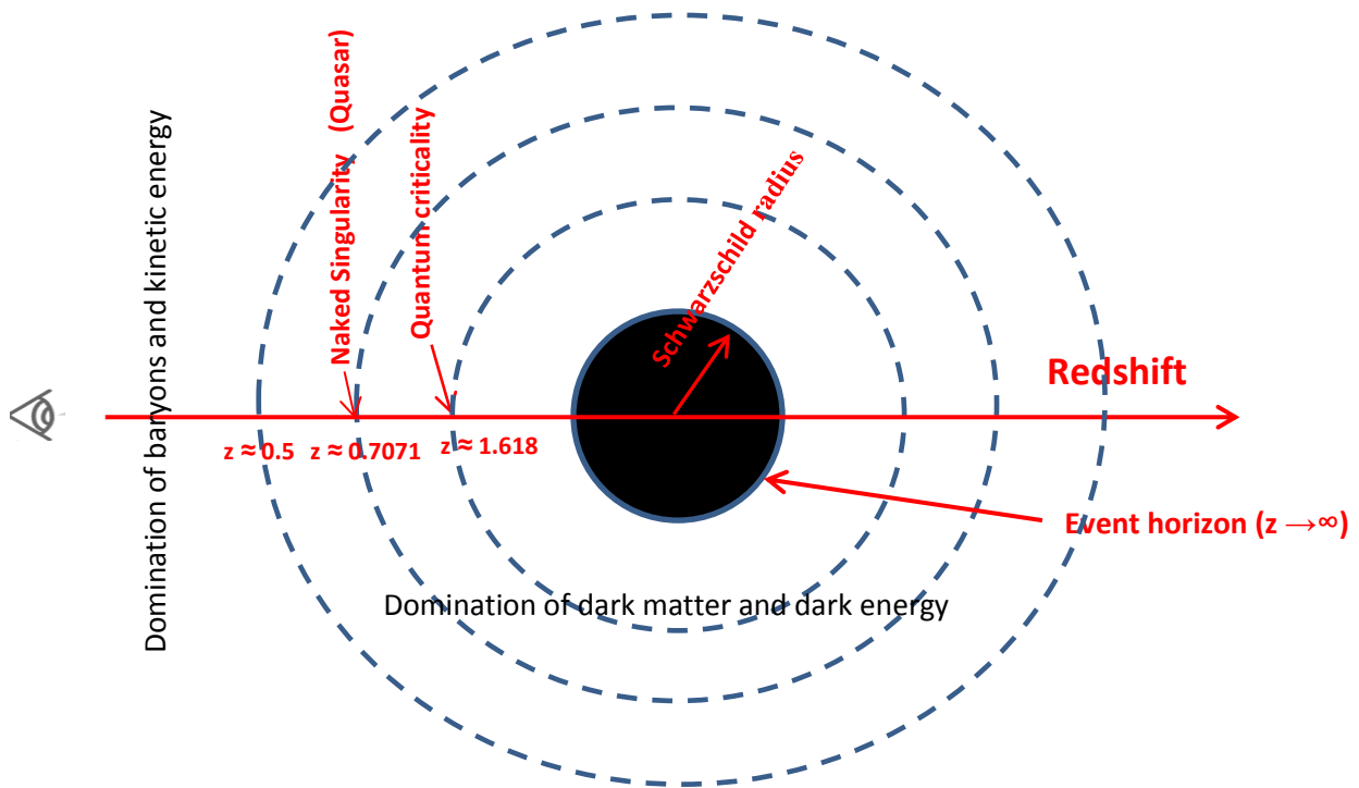
Figure 7 Illustration of the predicted black hole region
