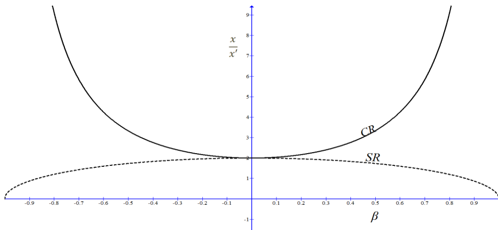
Figure a4: Distance transformation for the round trip. The dashed line depicts the corresponding prediction of SR
