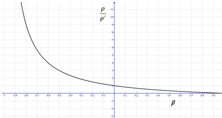
Figure a5. Mass density as a function of velocity
