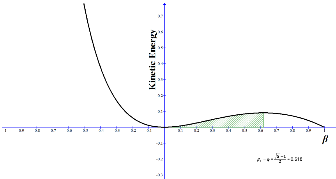
Figure a6. Kinetic energy as a function of velocity
