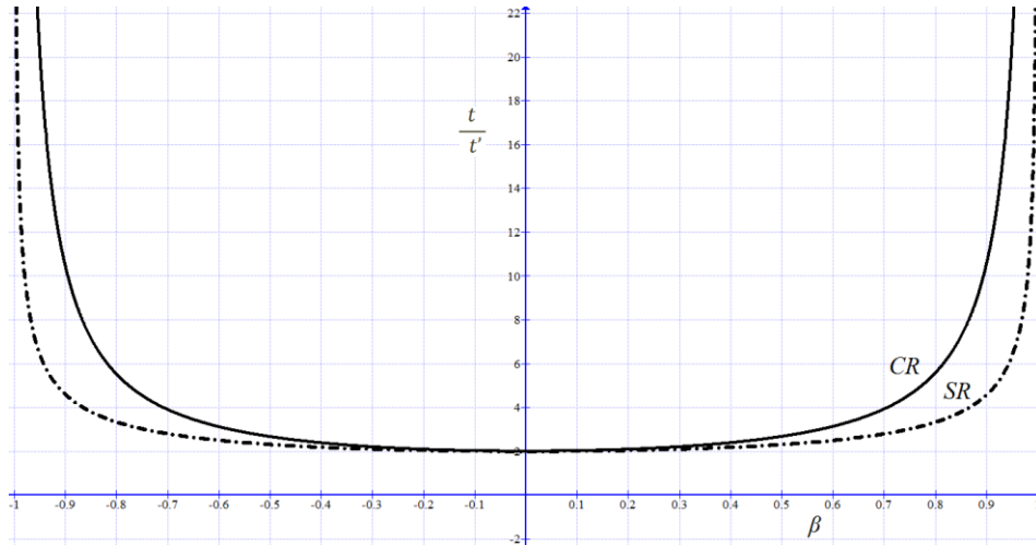
Figure a3. Time transformation for the round trip. The dashed line depicts the corresponding prediction of SR
