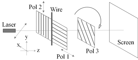
FIG. 1. Typical setup for the Quantum Eraser. Pol1 and Pol2 are fixed linear polarizers with polarizing axes perpendicular (x and y). Pol3 is a revoluble linear polarizer.
