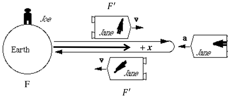
Figure 1. Twin Paradox
