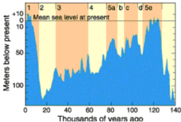
Late Quaternary sea-level history
