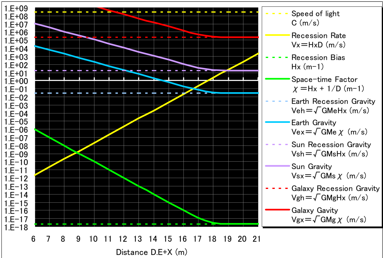
Fig.1. Relations of distance and each speed in the gravisphere
