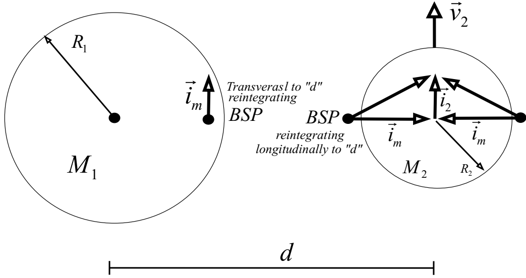
Figure 14: Ampere gravitation
