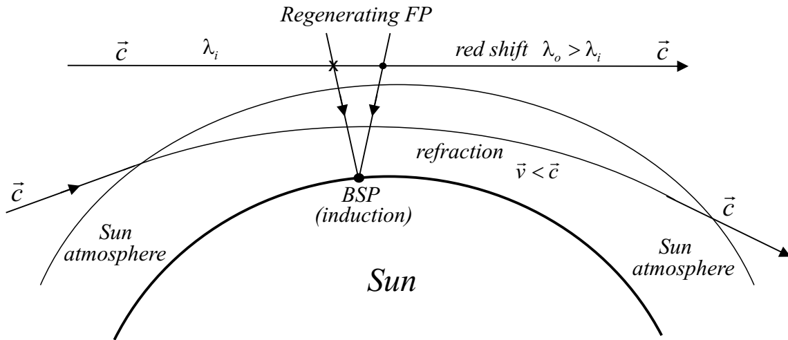
Figure 25: Refraction and red-shift at the Sun
