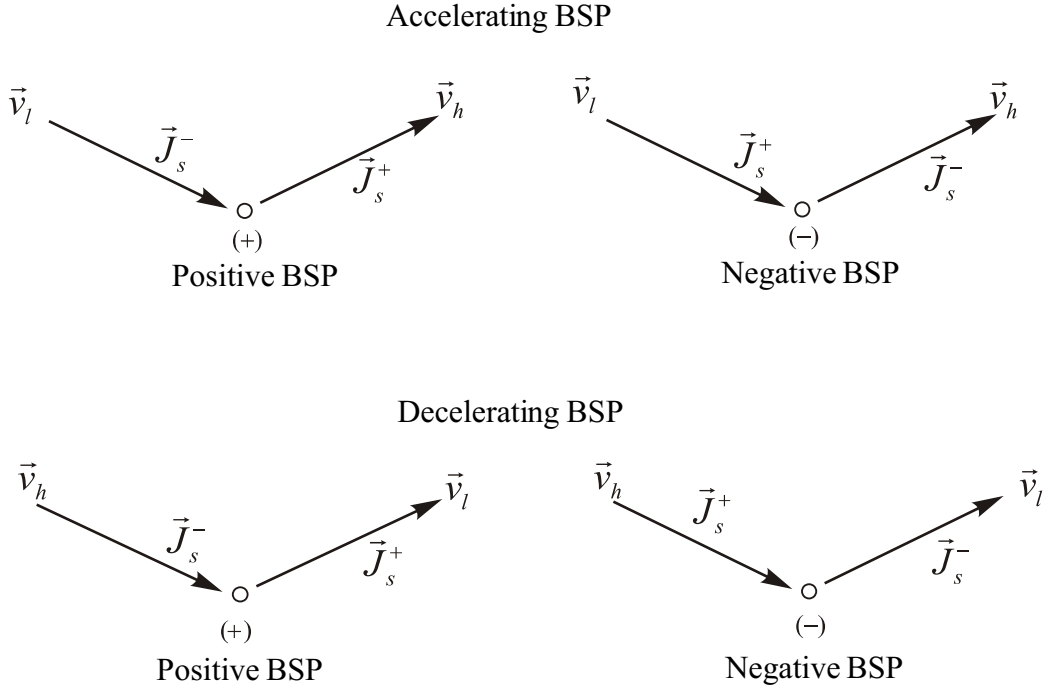
Figure 17: Conventions for BSPs
