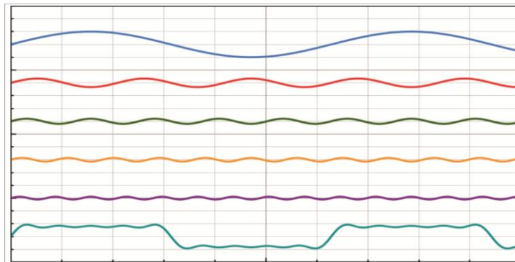
Fig.3: Graphs of spectral-components \sin(x) , \sin(3*x)/3 , \sin(5*x)/5 , \sin(7*x)/7 , \sin(9*x)/9 and their superimposition: \sin(x)+\sin(3*x)/3+\sin(5*x)/5+ \sin(7*x)/7+ \sin(9*x)/9 forming a 'gate-function'. All components are at the same phase 0^\circ at the origin x=0 , but they are at different phase-angles at different values of x .
