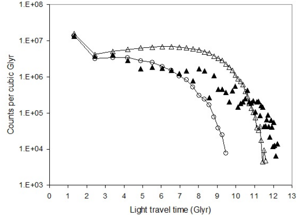
FIG. 3. Galactic density curve for Expanding Cosmology A, where Glyr are billion light years. The solid triangles indicate densities based on the zCosmos survey. The open dots indicate densities obtained by Monte Carlo simulation with a galactic radius of 78,000 light years. The open triangles are the simulated densities obtained with a galactic radius of 48,000 light years.
