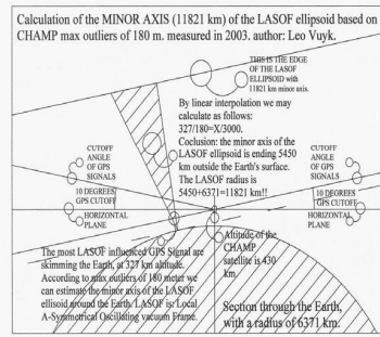
Calculation of the MINOR AXIS (11821 km) of the LASOF ellipsoid based on CHAMP max outliers of 180 m. measured in 2003. author: Leo Vuyk.
