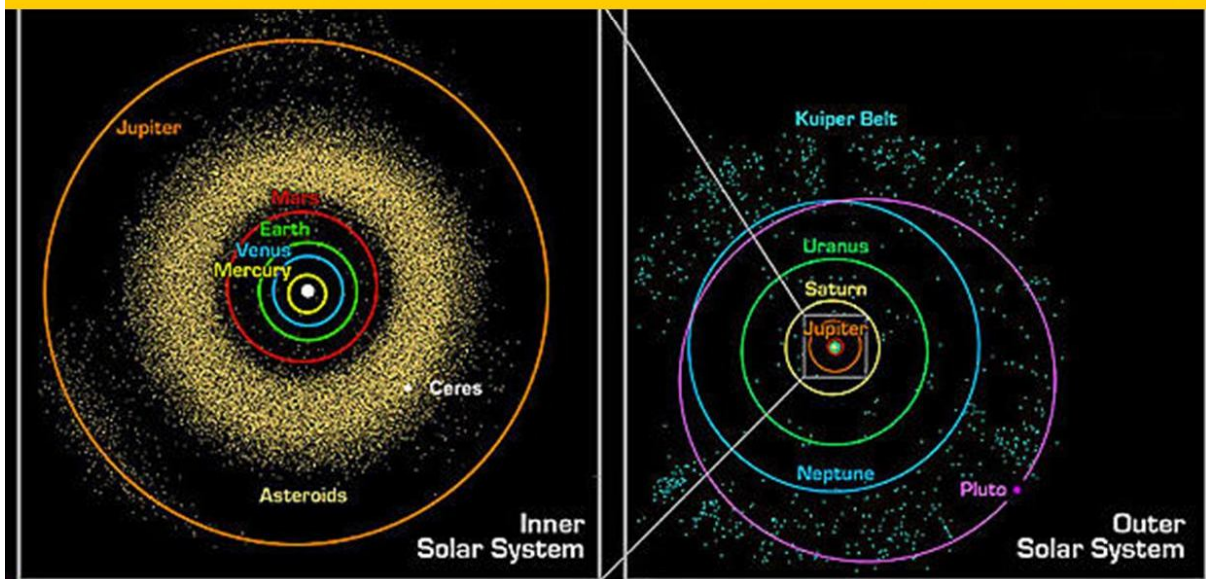
Figure: 22, Micro black hole based Comets produce H 2 and Water molecules building the icy Comet nucleus, spouting icy dust tails. Semi-Stationary Cometary objects ( P2013 P5) should be located all over the solar system, in the Oort cloud, the Kuiper belt and inner astroid belt, according to Quantum FFF Theory.
