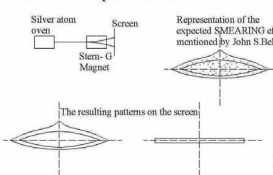
The screen pattern with the S-G magnet ON. The screen pattern with the S-G magnet OFF.
