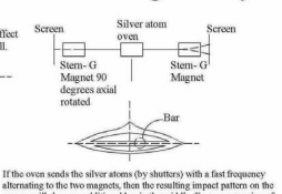
If the oven sends the silver atoms (by shutters) with a fast frequency alternating to the two magnets, then the resulting impact pattern on the screen, will show an additional bar in the middle. Even no smearing of impacts in between is supposed to show up, because of the absence of intermediate polarized atoms between 0 and 90 deg.
