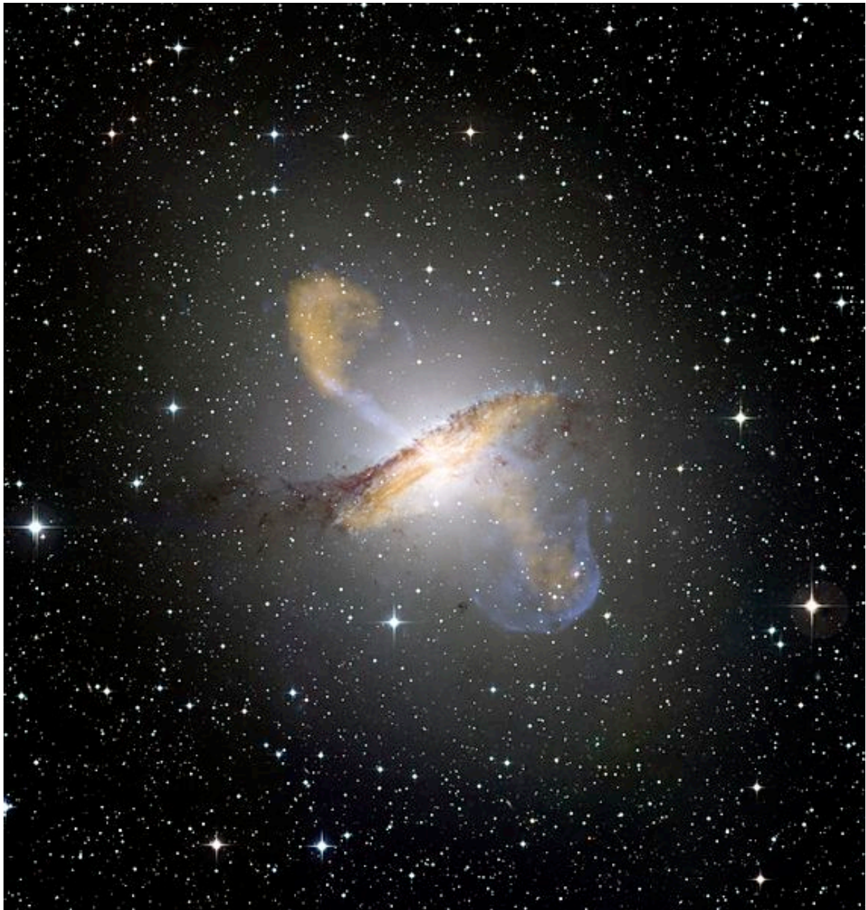
Figure 3. Centaurus A (NGC 5128), Credit: 'NASA/IPAC Extragalactic Database'.
