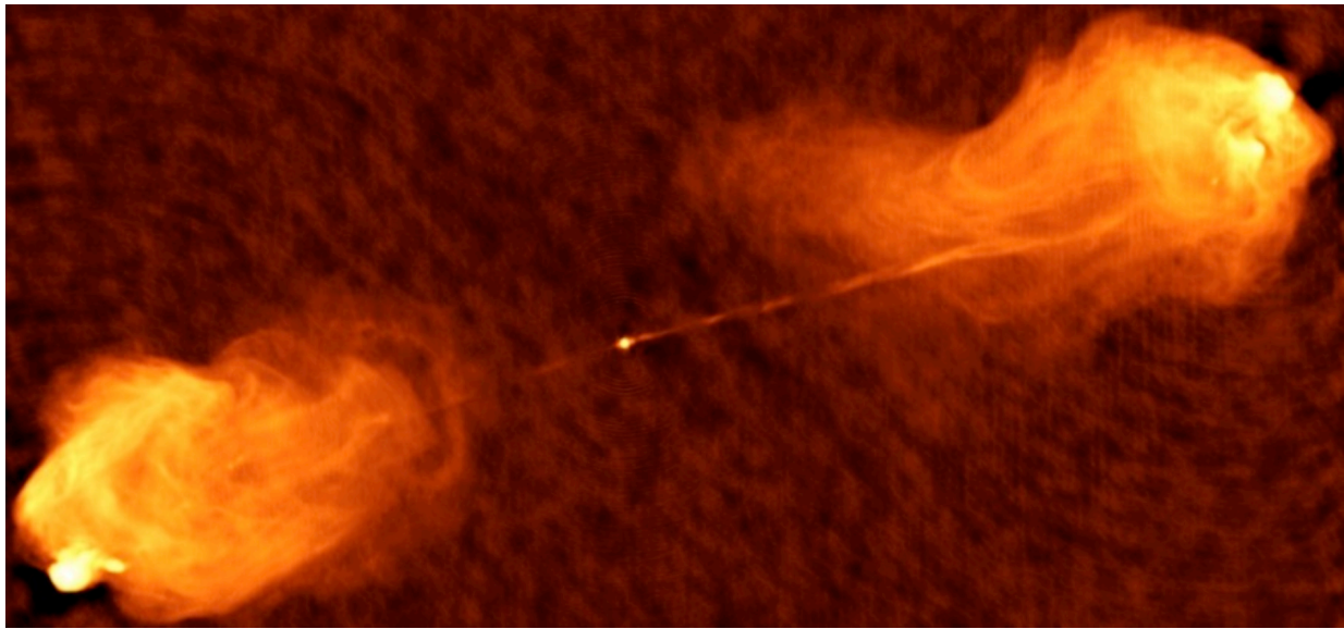
Figure 2. Cygnus A (3C 405), Credit: NRAO/AUI
