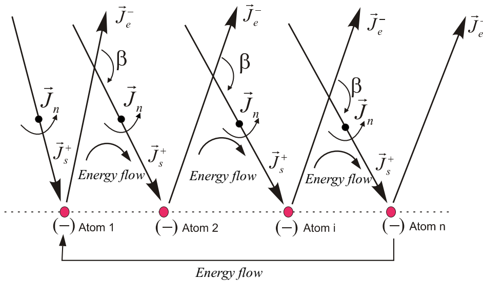
Figure 12: Energy flow along a closed chain of static basic subatomic particles
