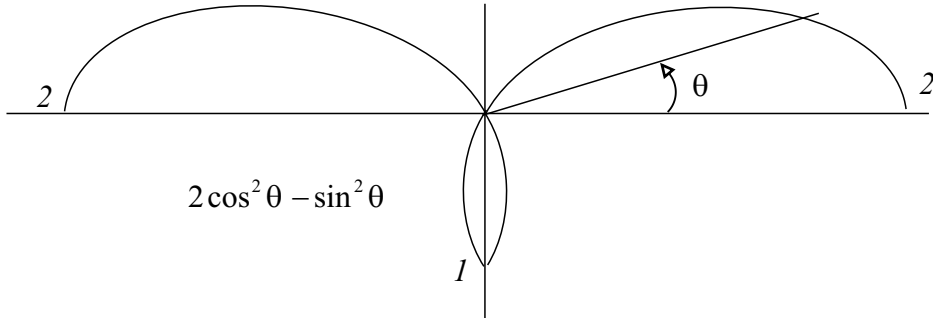
Figure 18: Plotting of the trigonometric relation for the analysis of Dragging.
