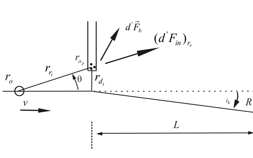
Figure 17: Force induced on a BSP at a bending edge by a BSP moving with speed v .
