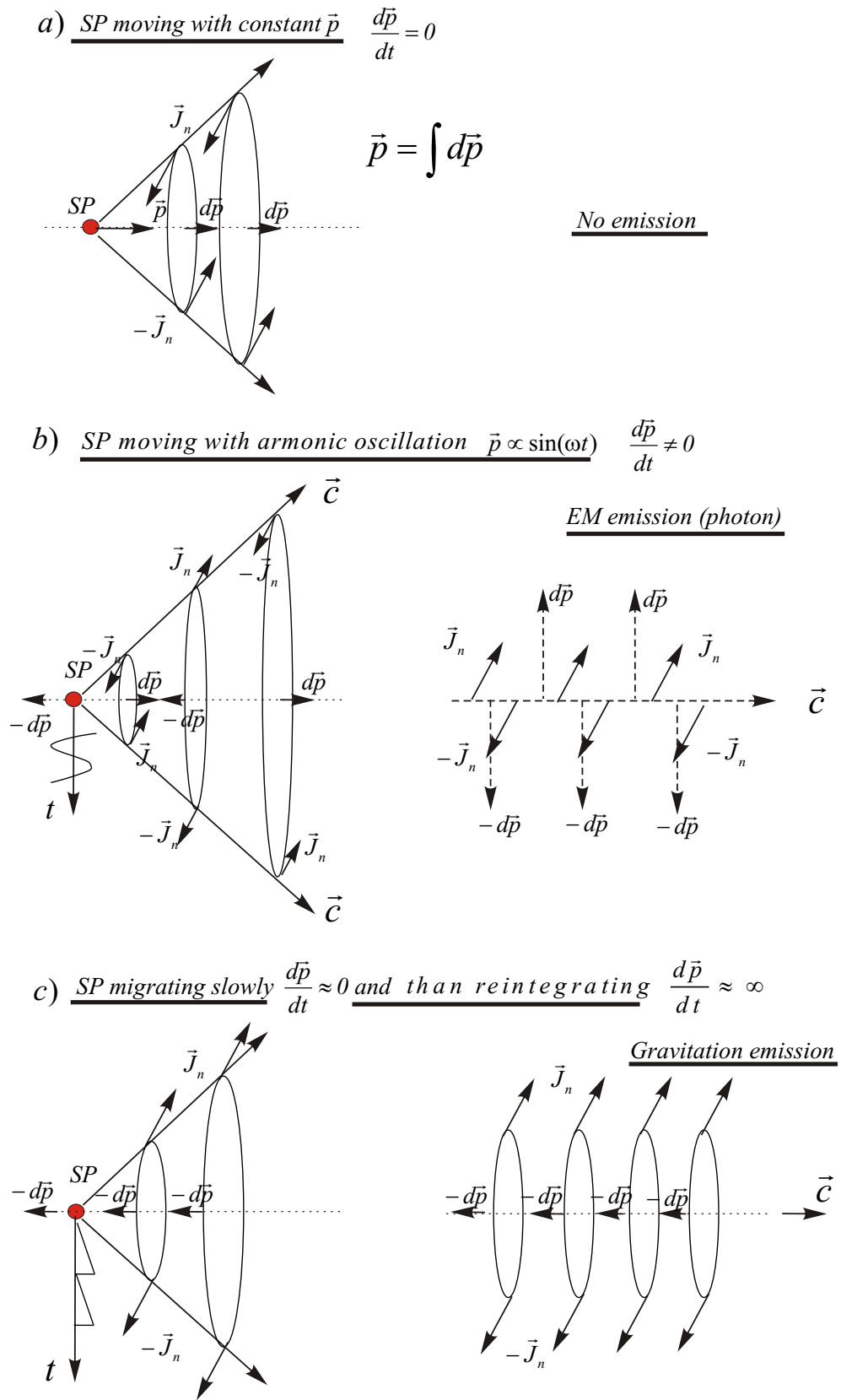
Figure 10: Electromagnetic and Gravitation emissions
