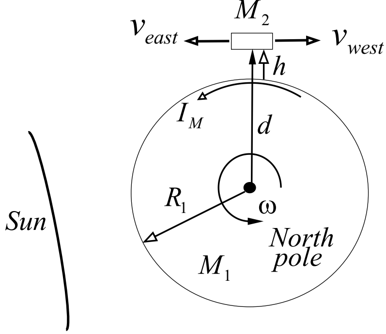
Figure 21: Influence of gravitation on clocks frequency.
