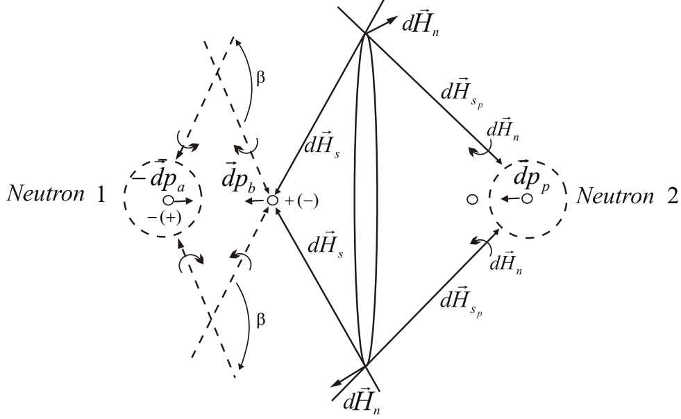
Figure 4: Transmission of momentum dp_b from neutron 1 to neutron 2
