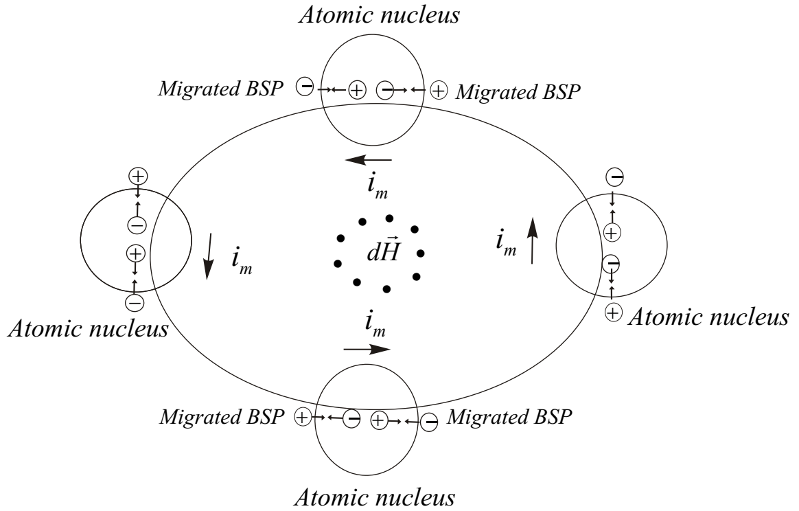
Figure 13: Current flow along a closed chain of reintegrating BSPs
