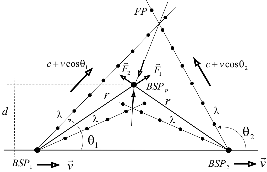
Figure 19: Dragging due to Doppler effect.
