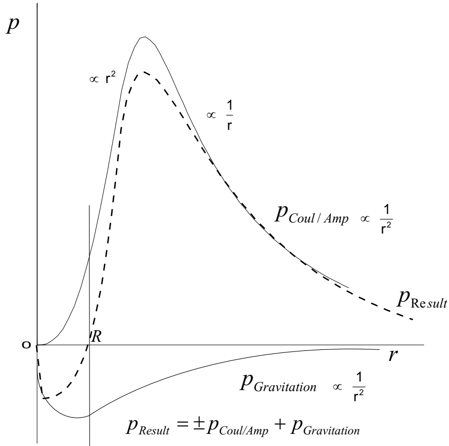
Figure 9: Resulting linear momentum p due to Coulomb/Ampere and Gravitation momenta.
