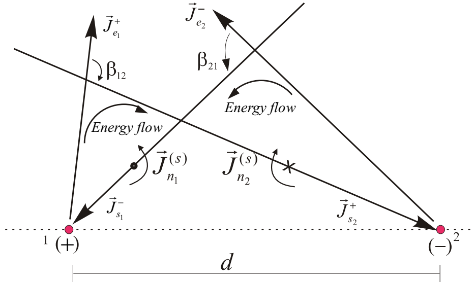
Figure 11: Energy flow between two static basic subatomic particles
