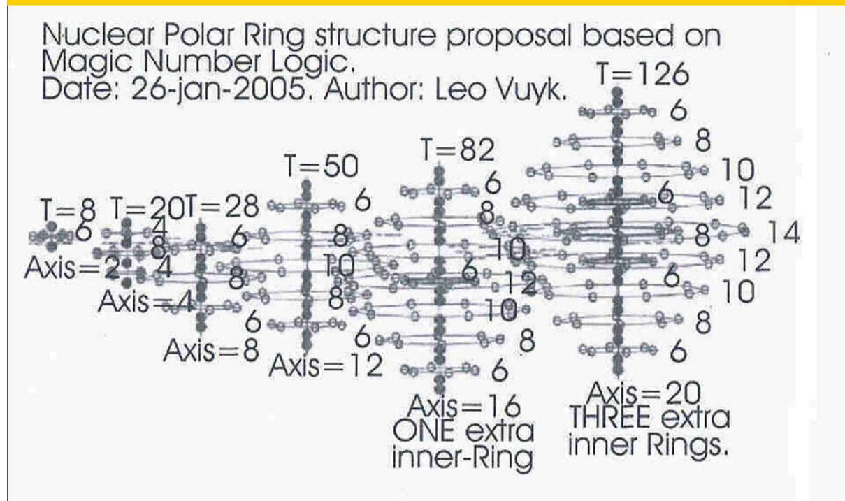
Figure: 3, different view on 3D nuclear polar coaxial ring structure without the T=34 structure (for clarity).
