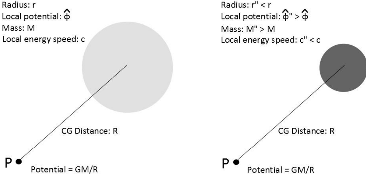
Fig 2: When a sparse spherical body is compacted into a denser spherical body, the local gravitation potential of all contained matter and energy increases. This is equivalent to an increase in mass, but that cannot result in an increase in potential at a distance location P, as the total gravitational energy does not increase. The increase of mass is compensated by a reduction of energy speed or a red shift of all constituent energy (including gravitational energy) so that the potential at P remains the same.
