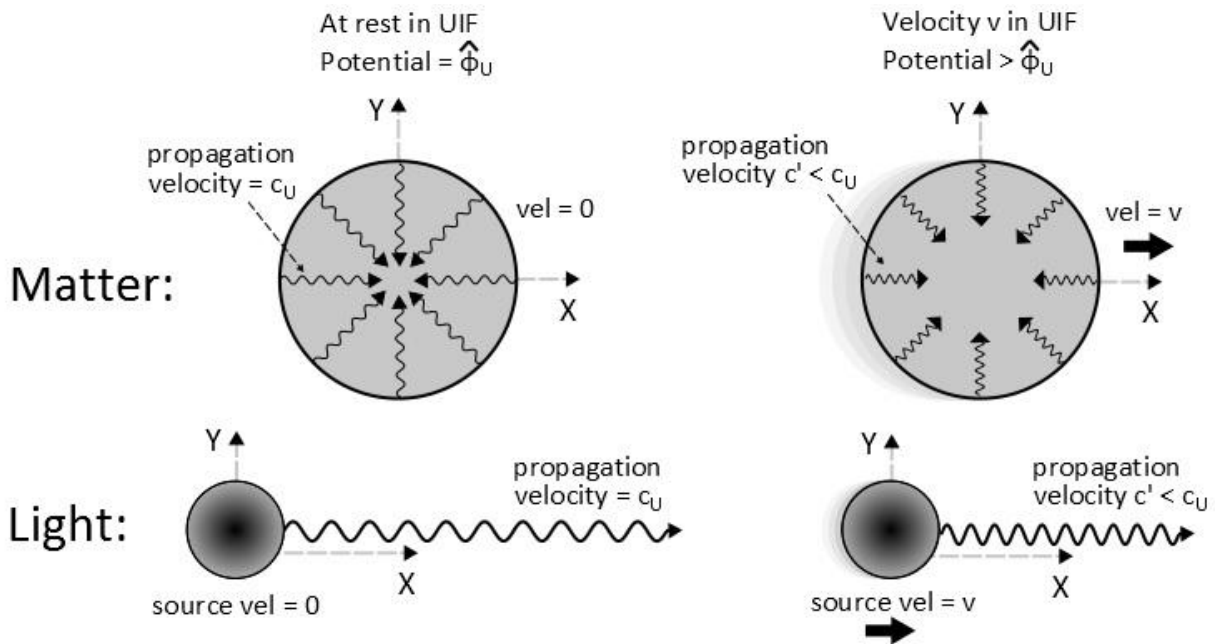
Fig 4: Effect of changed potential on velocity of matter and light/ energy is different. When a body of matter moves at a velocity v in UIF, energy propagation velocity within it is slowed down in all
