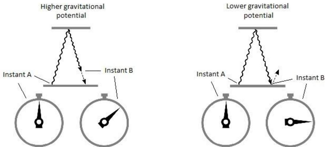
Fig 1: The light clock and mechanical clock on the left are in a higher gravitational potential than the light clock and mechanical clock on the right. Light and all energy moves slower in the left side configuration. At instant A, both sets of light and mechanical clocks are synchronized. At a later instant B, the readings on the left side clocks will fall behind the right hand one, as light in the light clock and all energy within the mechanical clock on the left are traveling proportionately slower. The size of the 'second' in the left hand configuration is longer than the 'second' on the right hand side.
