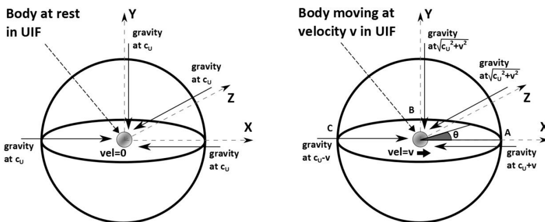
Fig 3: A body at rest in the UIF receives gravitational energy at c_U from all directions. When it travels with a velocity v in any direction (X-axis in the figure above), the gravity is blue shifted in the direction of motion and red shifted in the opposite direction, with intermediate values in other directions.
