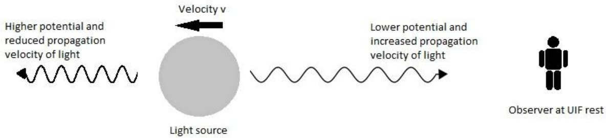
Fig 5: As the light source moves away from the observer, light emitted towards the observer faces lower potential, and therefore its propagation velocity increases. At normal light speed in UIF (i.e. c_U ), for a small velocity v , the negative speed of the light source is almost exactly compensated by the increase in propagation velocity, and the light speed appears unaffected to the observer at rest. This is the mechanism behind the 'invariance postulate'.
