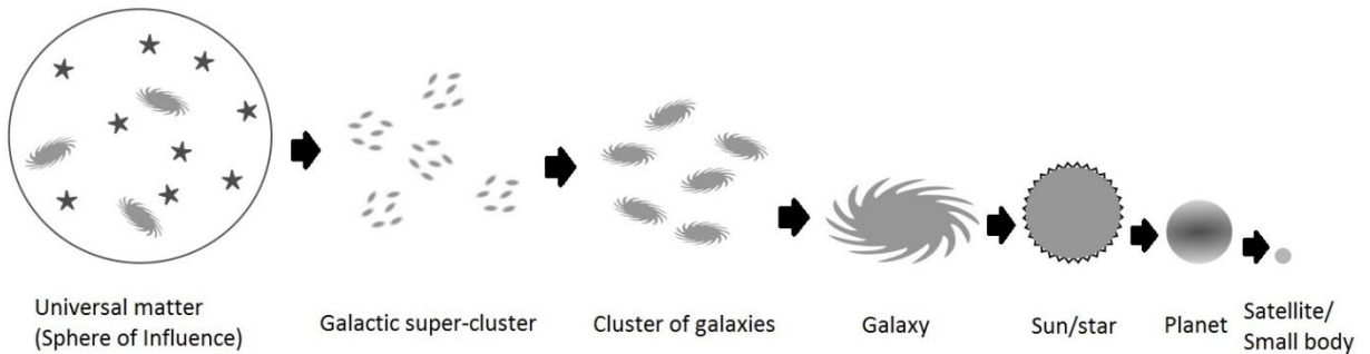
Fig 6: Objects higher in the hierarchy determine the potential of objects lower down the order. Since gravitationally bound systems (objects at any two successive levels – e.g. planet and satellite) are subjected to the common potential of all higher order objects (e.g. Sun/star upwards), the relative time dilation between such objects depend solely on the local mass distribution and velocities from the CG within the system.
