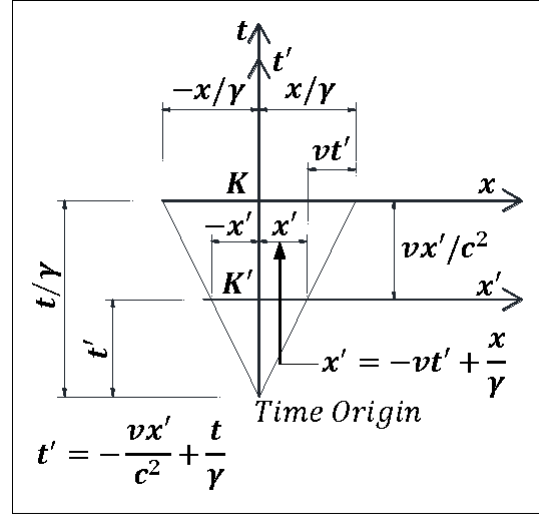
Fig. 2: Graphical representation of Lorentz transformation equations (2).
