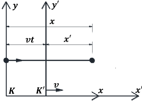
Fig. 3: x -coordinate with respect to K .
