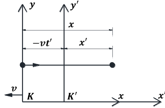
Fig. 4: x' -coordinate with respect to K' .
