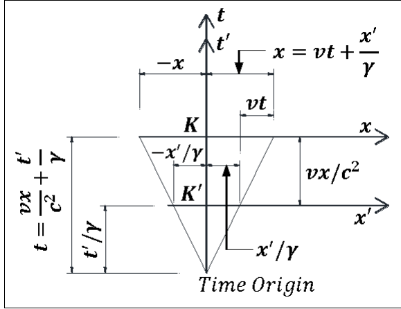
Fig. 1: Graphical representation of Lorentz transformation equations (1).
