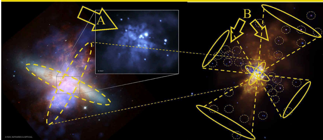
Figure 16, M82 Starburst Galaxy with a complex galaxy anchor black hole system
