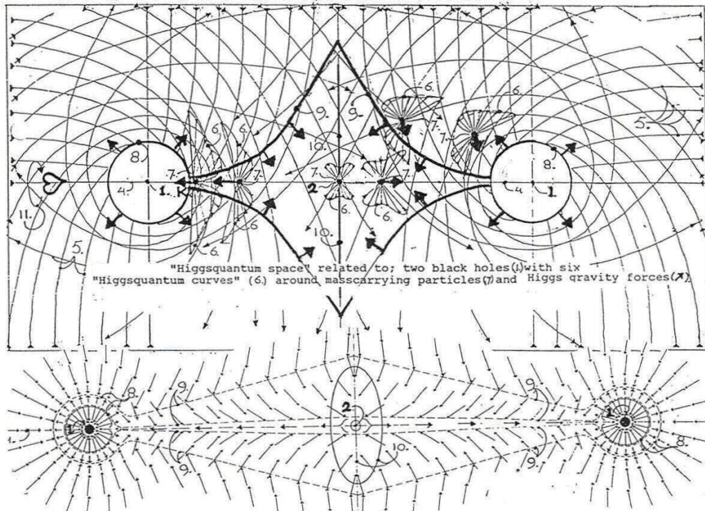
Figure 2, impression of the Higgs Vacuum structure around a set of two Black holes, as is found to be present around some Planetary nebula, early Galaxies and Herbig Haro objects. The negative charged particle jets is the result of the Black hole based electric potential combined with the vacuum polarisation (acceleration) effect on light Fermions like electrons and the origin of Birkeland currents and Alfvén circuits.
