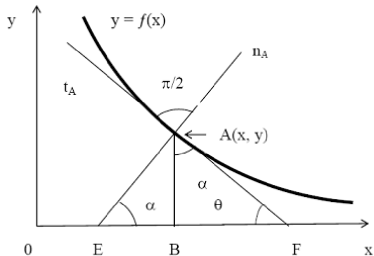
Figure 2. Rod deformation and Lobachevski function:
