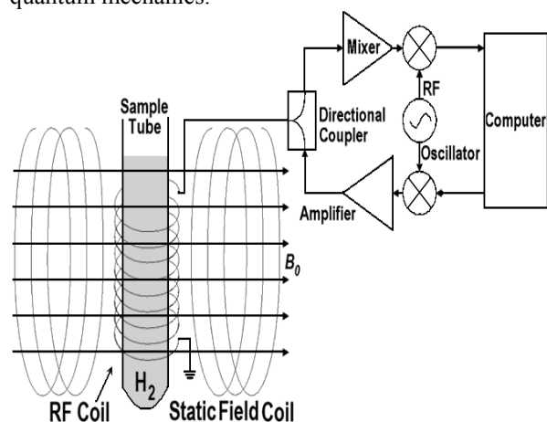
Figure 14. NMR apparatus designed to manipulate TBS in Hydrogen. The Fig. only shows possible details for rf-modulating TBS QED resonance, not the spectrographic recording and analysis components.
