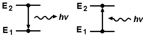
Figure 11. a) Decrease in energy level E2 to E1 resulting in photon emission (squiggly arrow) with quantized energy, \hbar\nu . b) An increase in energy level from E1 to E2 resulting from absorption of a photon (squiggly arrow) also with energy, \hbar\nu . This is the simplistic basis for spectrographic analysis of the quanta in a particular atomic orbit. The TBS experiment anticipates 3 new spectral lines in atomic hydrogen under the novel conditions set up by the apparatus.
