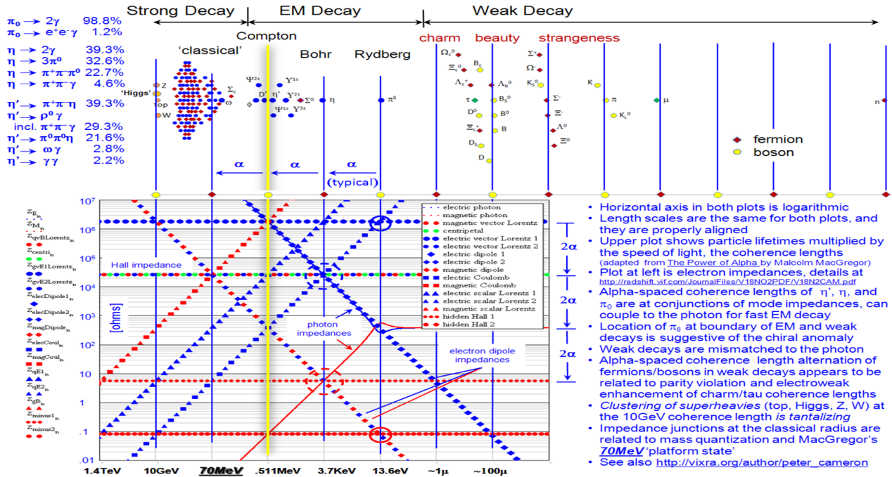
Fig. 1. Composite of 13.6eV photon [6] and background independent electron impedances [3], measured \pi_0 , \eta , and \eta' branching ratios, and unstable particle coherence lengths [7].
