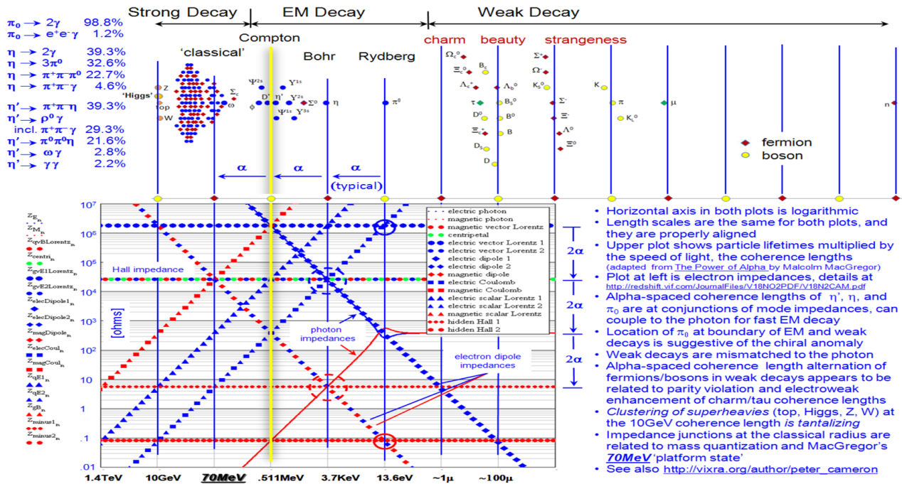
Fig. 1. Composite of 13.6eV photon [?] and background independent electron impedances [?], measured \pi_0 , \eta , and \eta' branching ratios, and unstable particle coherence lengths [?].
