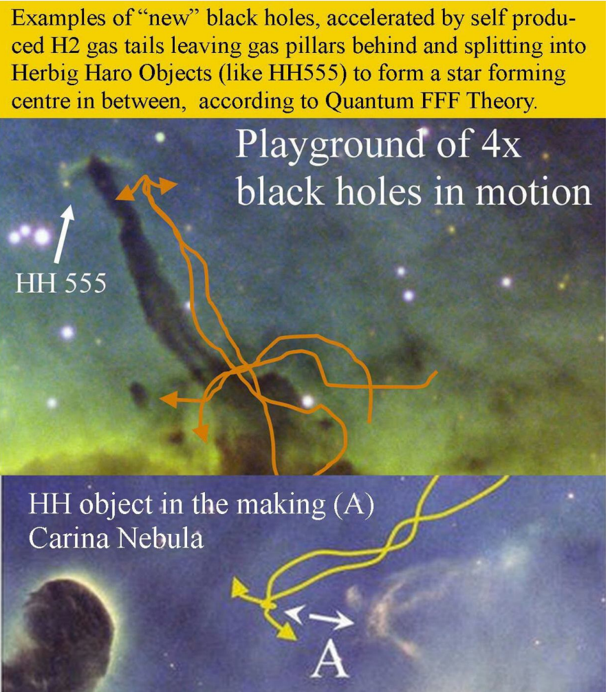
Figure 12, Pairing and splitting new oaradigm black holes the origin of gas pillars HH objects and Bok globules.
