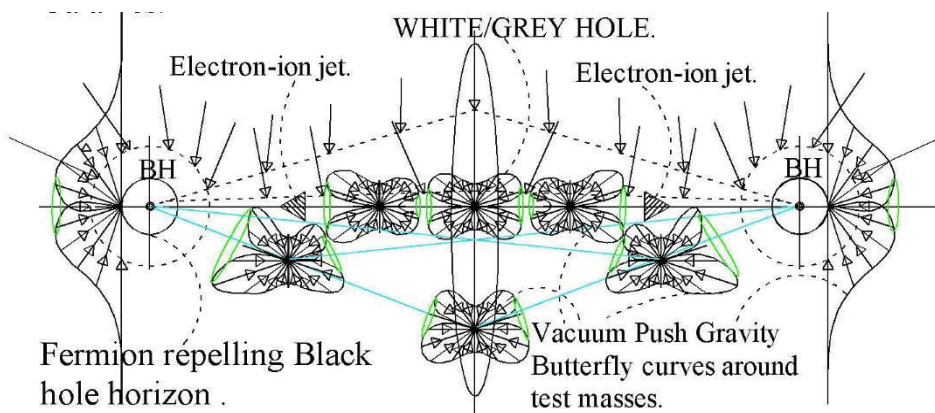
Figure 4, The same Birkeland current system as figure 3 with butterfly vector arrays at different locations around the Black holes. In the middle the vacuum has less density ( larger Planck lengths) by the absorption of the dual Black holes.
