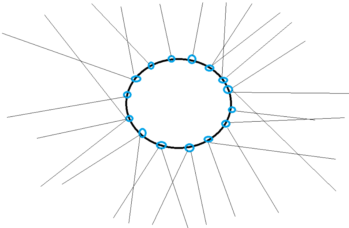
Figure 15. Star. Excess object is ejected when these flow merger to become a giant circularflow called a star.
