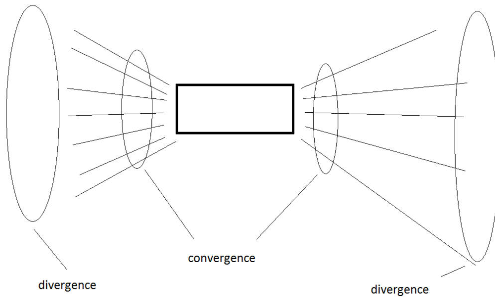
Figure 19. Distribution of vortices close to permanent magnet.
