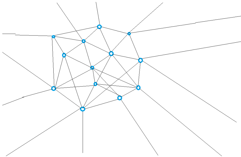
Figure 13. Cloud of atoms trapping flows.
