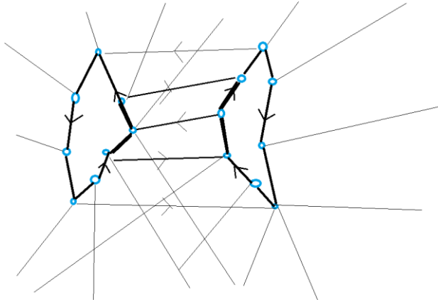
Figure 14. Electric Flows involved in hydrogen cloud.
