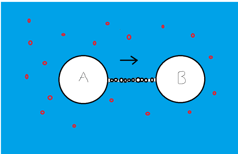
Figure 11. Atom moving from position A to position B.
