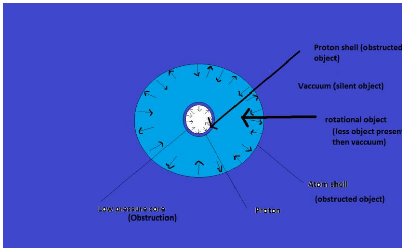
Figure 31.Cone model of hydrogen.
