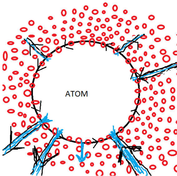
Figure 18. Push on the atom.
