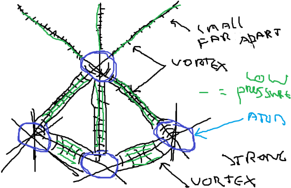
Figure 1. is greatly exaggerated in order to visualize. Atoms are a build of gazillions of small vortices.Magnetic circular flow gets just a little bigger when cones get closer. This causes lower pressure "under" the atom then above causing an acceleration of the atom.
