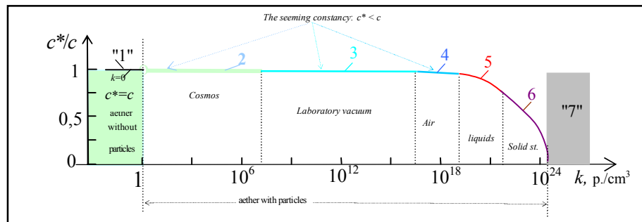
Fig.1. By understanding the seeming "independence" of the speed c^*=(\epsilon\mu)^{-1/2} , the propagation of EMW from the concentration ( k, p/cm^3 ) particles of vacuum and gases atmospheres in the simplest linear scale representation of the vertical axis c^*/c=n^{-1} , where n – the index of refraction, in which propagation EMW ( n^2=\epsilon\mu/\epsilon_0\mu_0 ).
