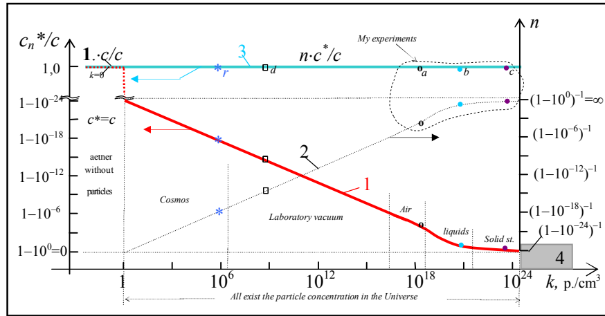
Fig.2. Stretched by double logarithmic scales of abscissa axis ( k ) and ordinates \{c_n^*(k)/c and n\} of dependencies: 1 – of relative velocity c_n^*(k)/c propagation EMW; 2 – of the refractive index n(k) , where k – concentration of particles (or polarizing atoms) under atmosphere nonmoving IRS 0 . Constant level 3 is the product of the corresponding values of curves 2 and 1; he determines actual invariant \{n \cdot c^*/c\} of ADTR.
