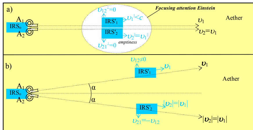
Fig.3. The proof due to experiments on accelerators of relativistic particles (muons and pions) fallibility of Einstein kinematic interpretation TR:
