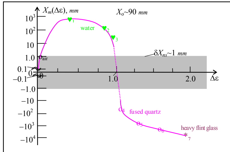
Fig.4. Dependence of the amplitude X_m of the harmonic shift of the interference fringe from the contribution \Delta\varepsilon of particles in full dielectric permeability \varepsilon=1+\Delta\varepsilon of optical media (air, water, fused quartz, heavy flint glass) from [13 1 ].
