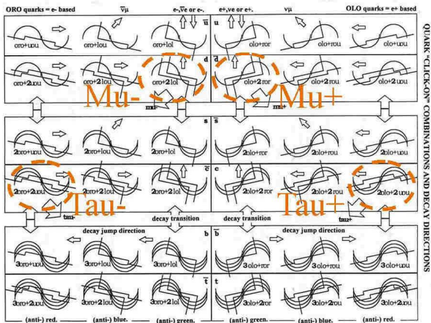
Figure 17, Sub Quantum structure proposal for elementary particles of the standard model.
