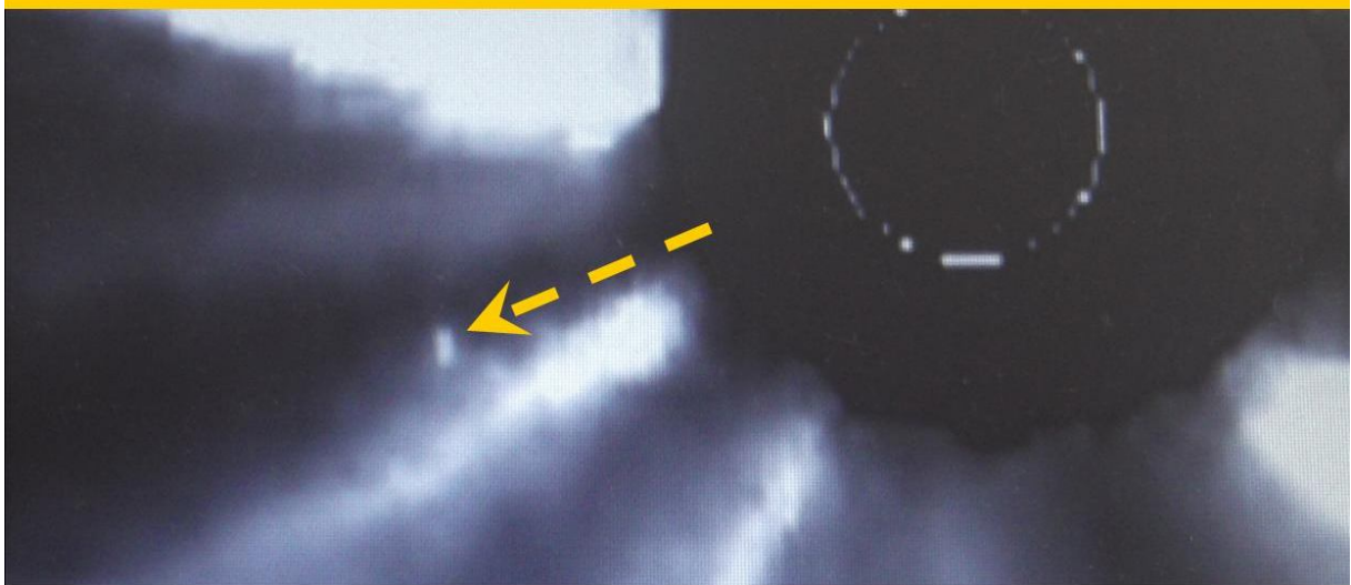
Figure 23, Assumed creation of Quantum Knot based Black Holes by electro magnetic interference (knitting) effects. (See figure 6)
