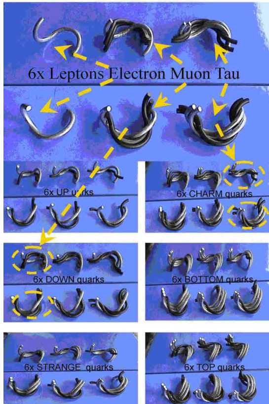
Figure 17, Sub Quantum structure proposal for elementary particles of the standard model.
